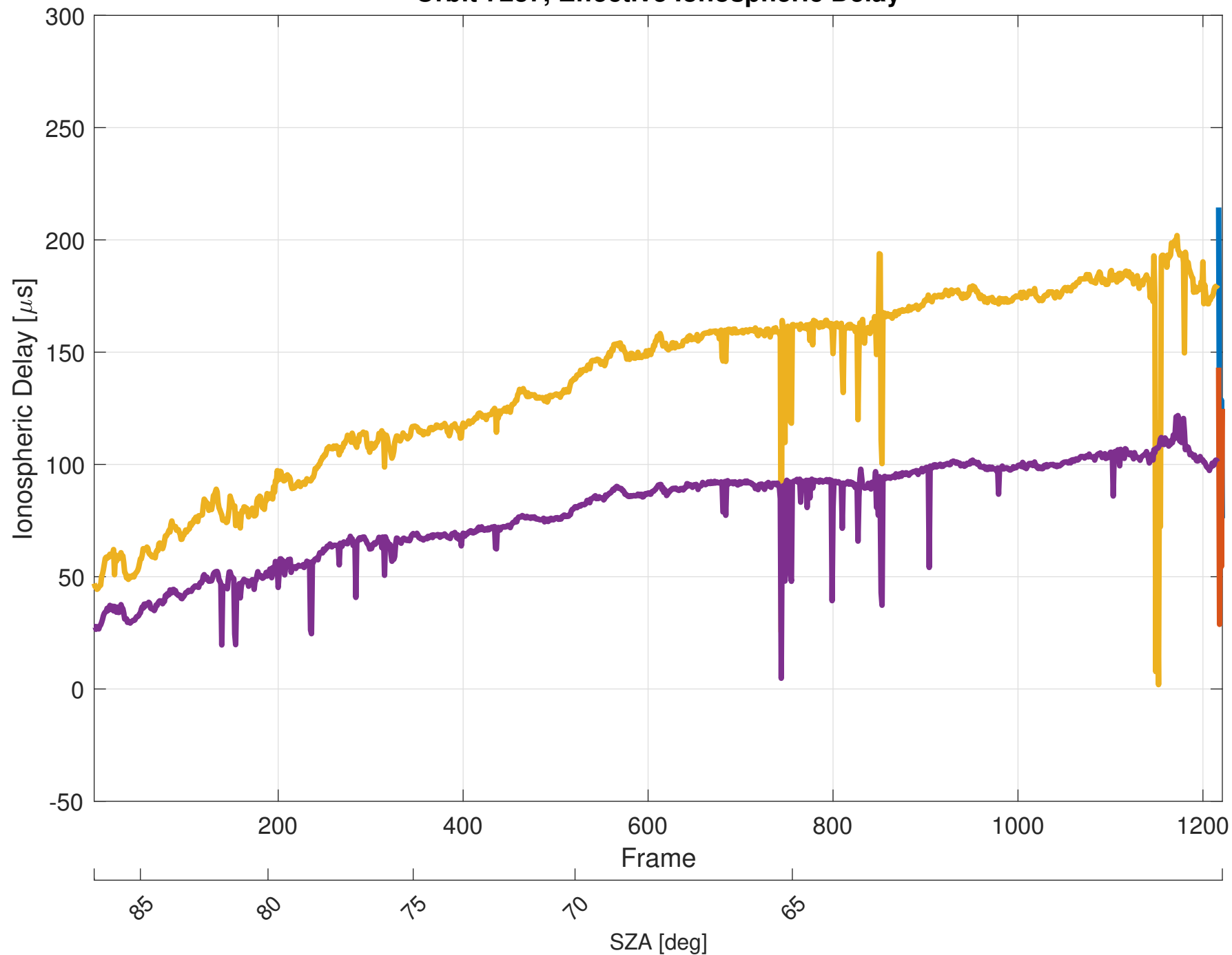
Orbit 7237, Effective Ionospheric Delay
