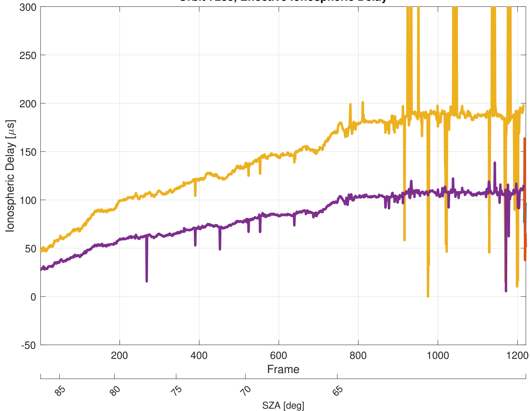
Orbit 7238, Effective Ionospheric Delay
