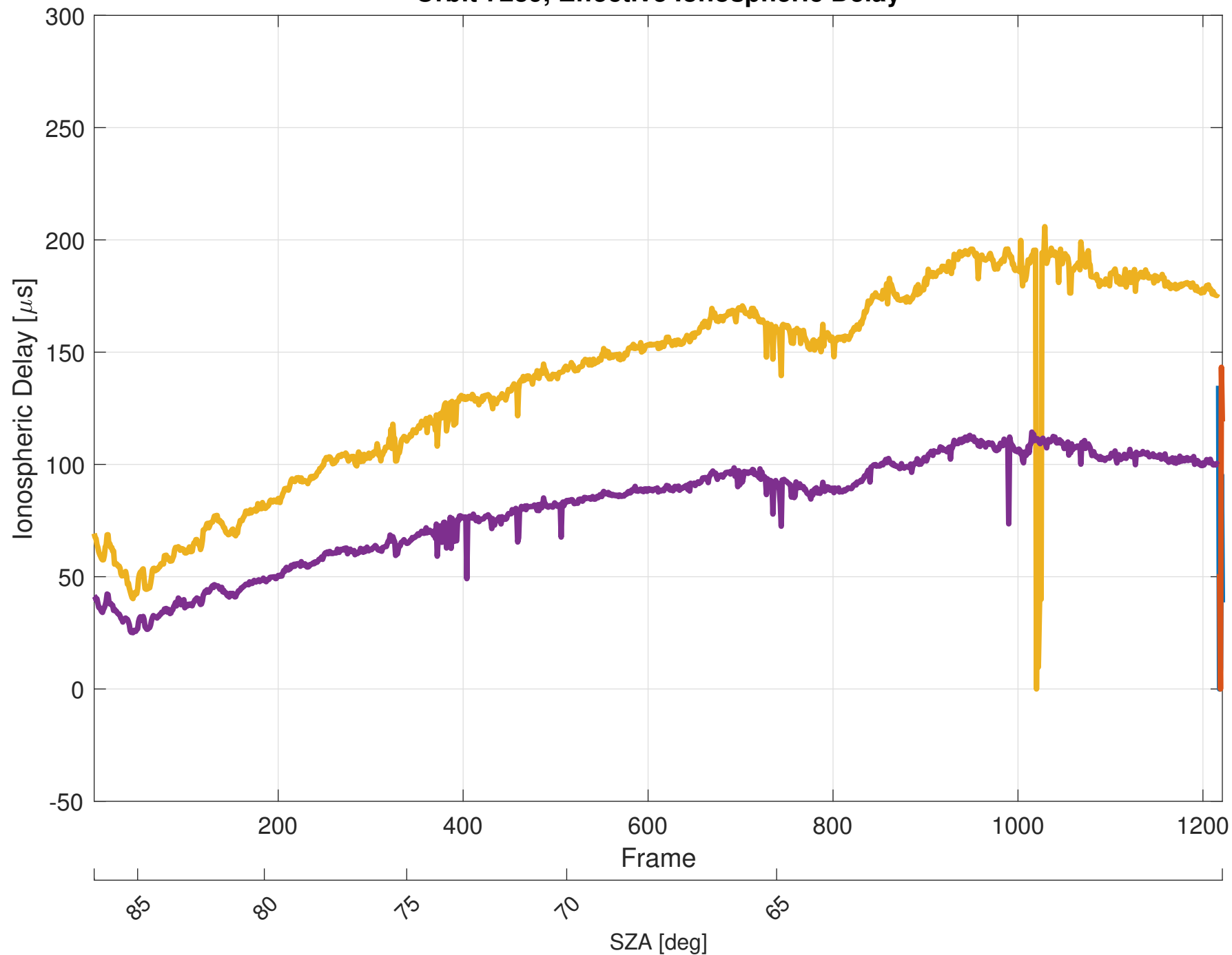
Orbit 7239, Effective Ionospheric Delay
