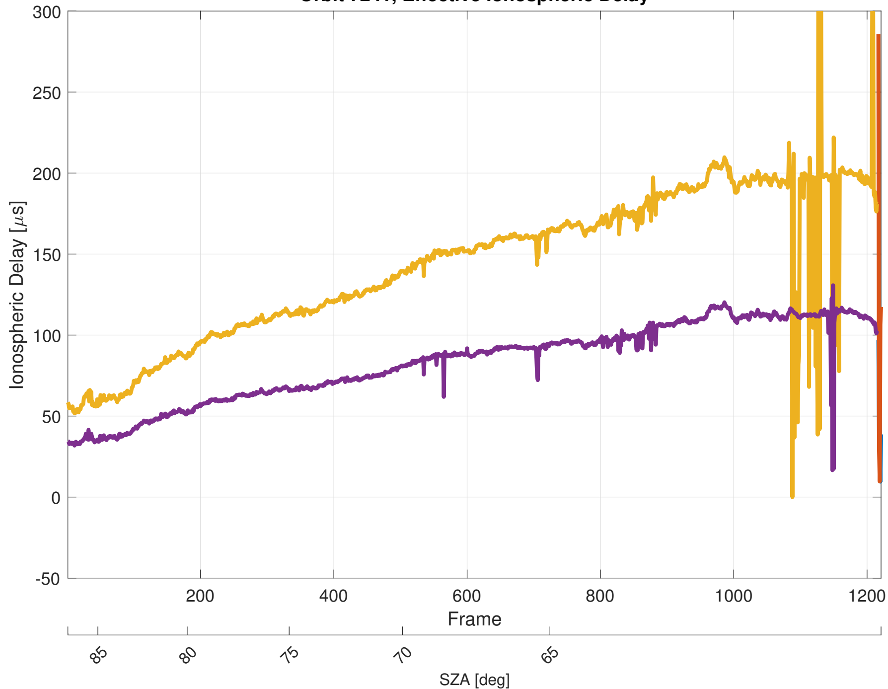
Orbit 7241, Effective Ionospheric Delay
