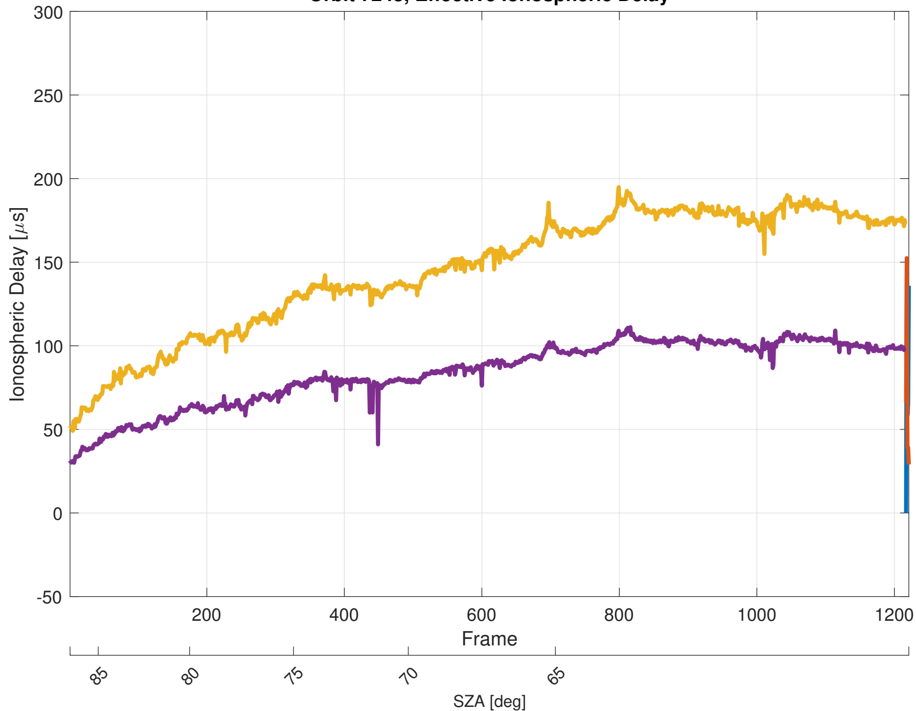
Orbit 7243, Effective Ionospheric Delay
