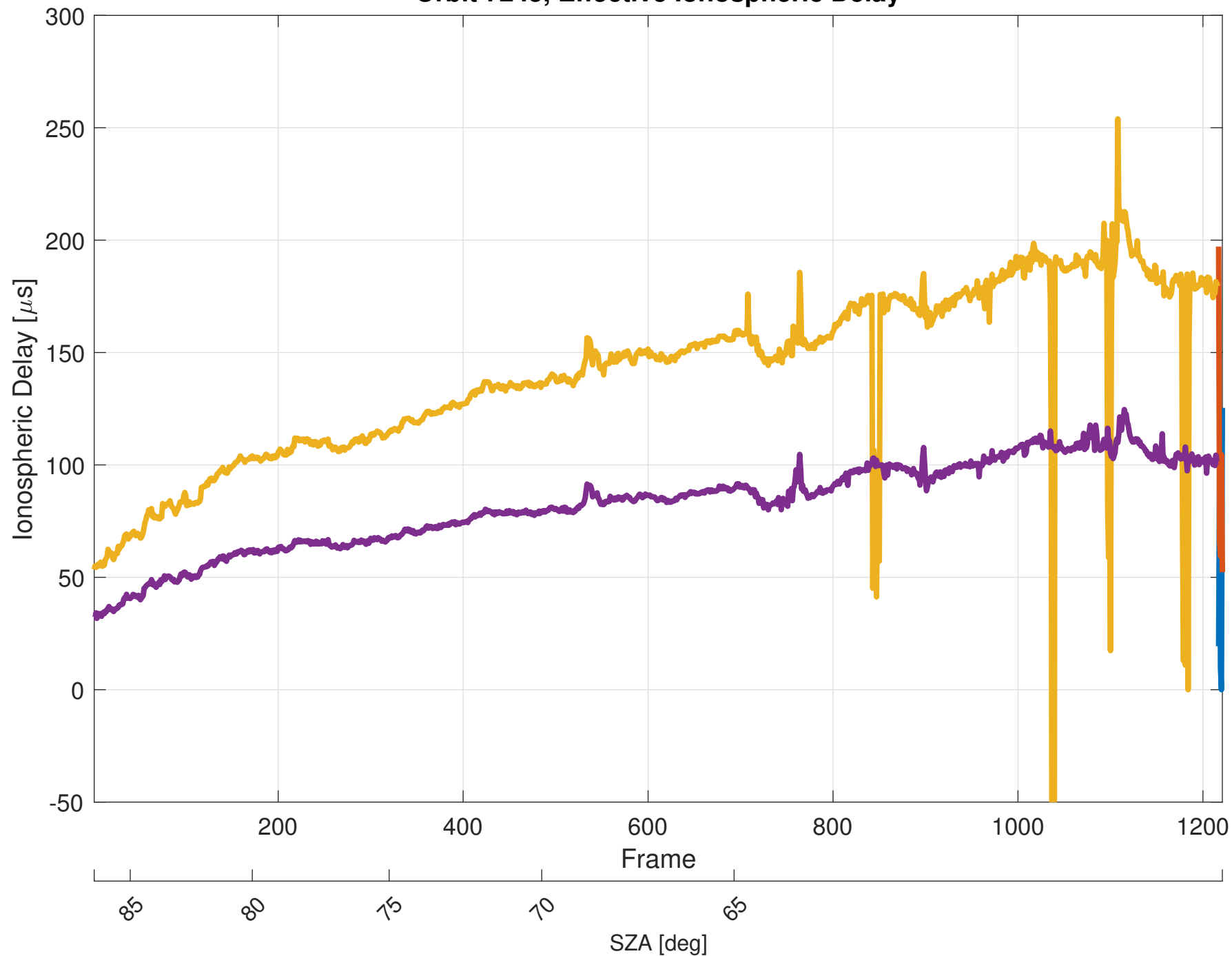
Orbit 7245, Effective Ionospheric Delay
