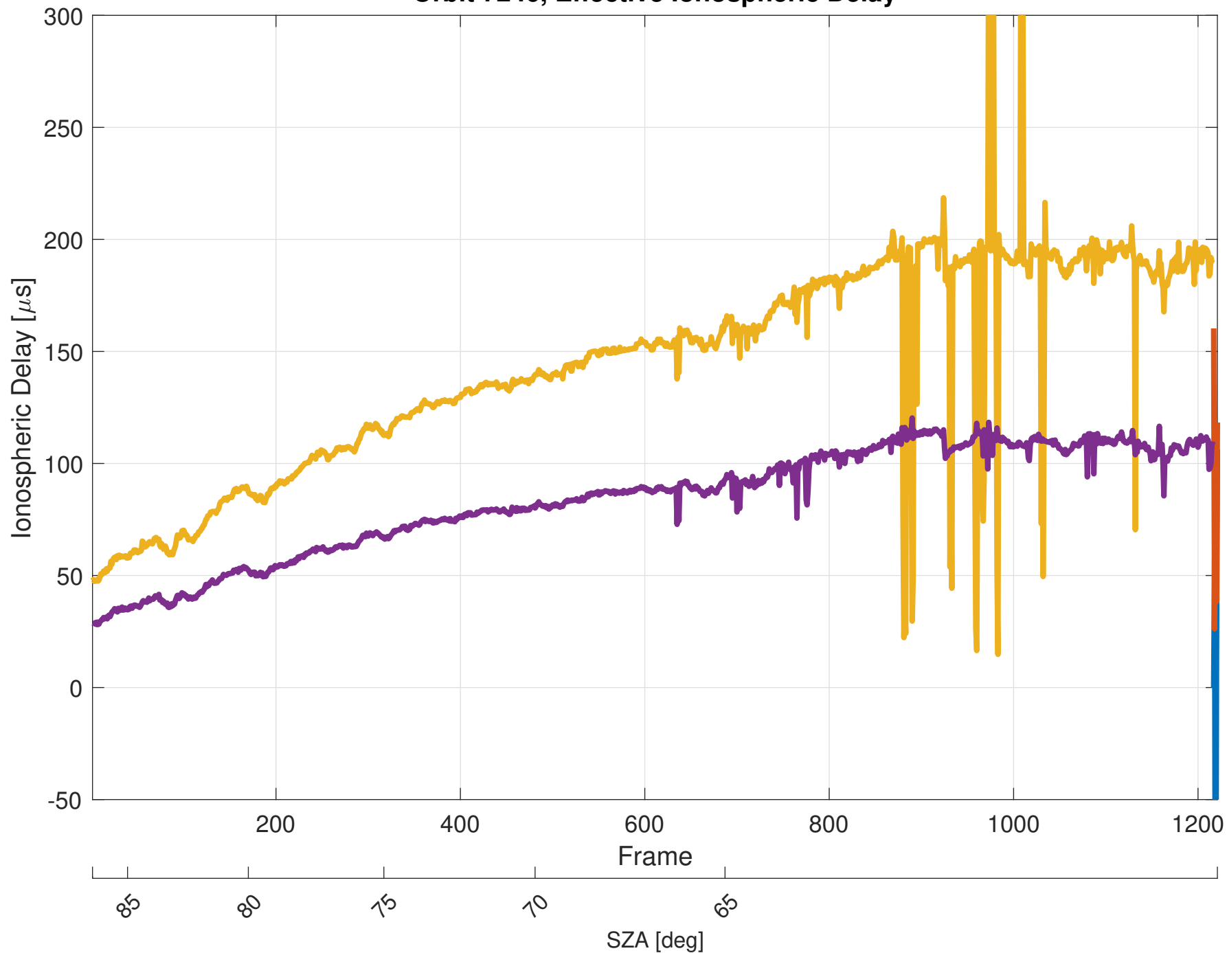
Orbit 7246, Effective Ionospheric Delay
