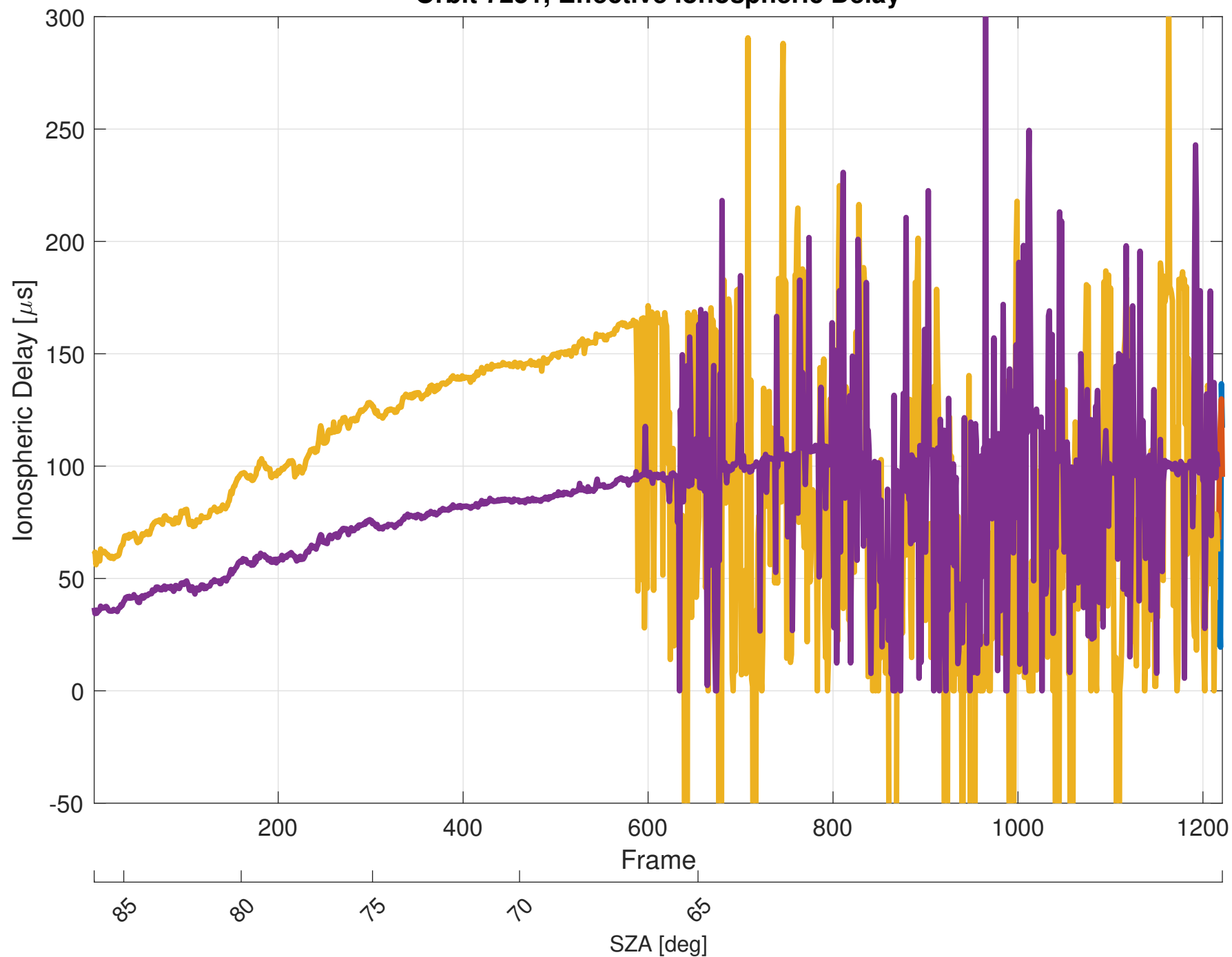
Orbit 7251, Effective Ionospheric Delay
