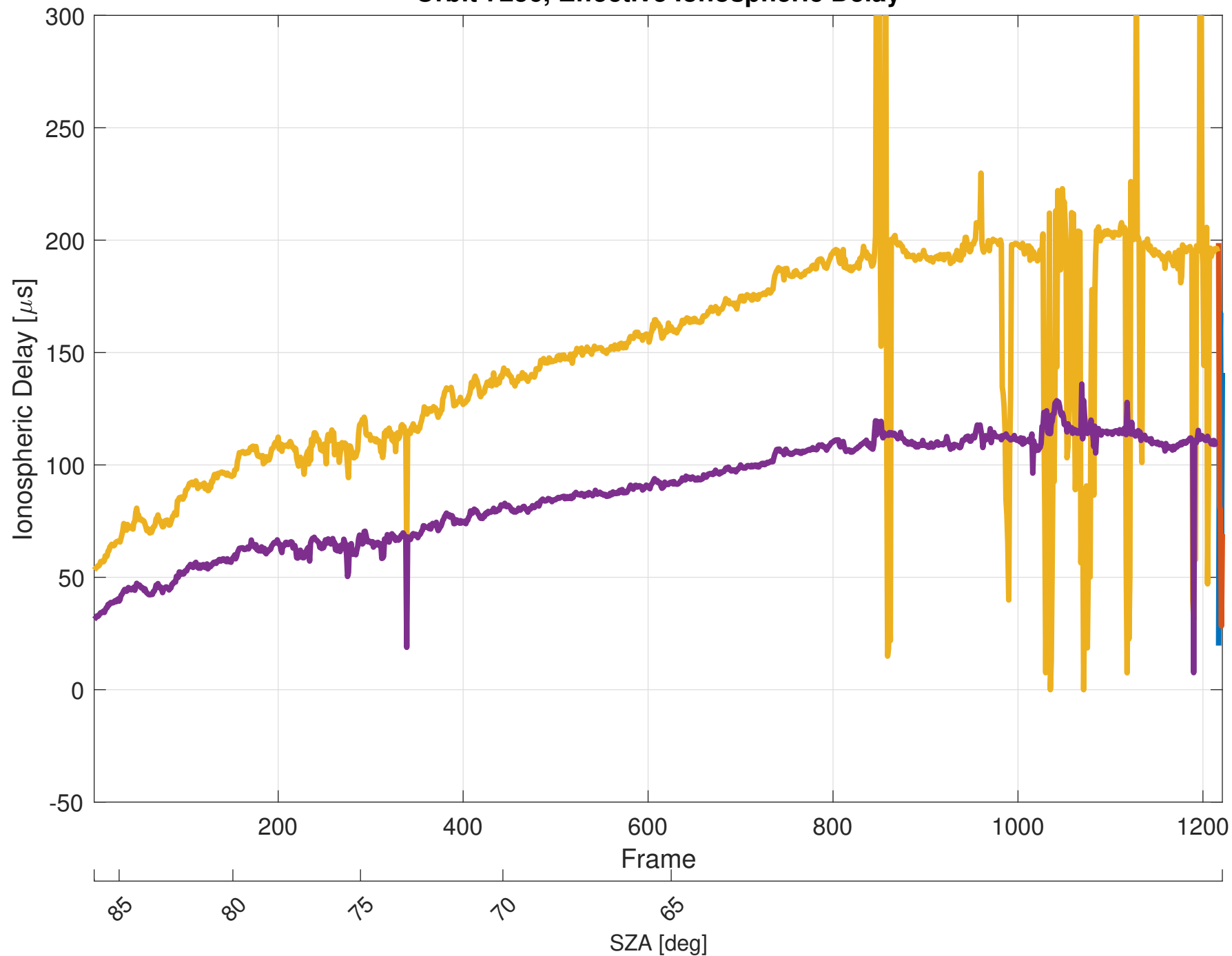
Orbit 7256, Effective Ionospheric Delay
