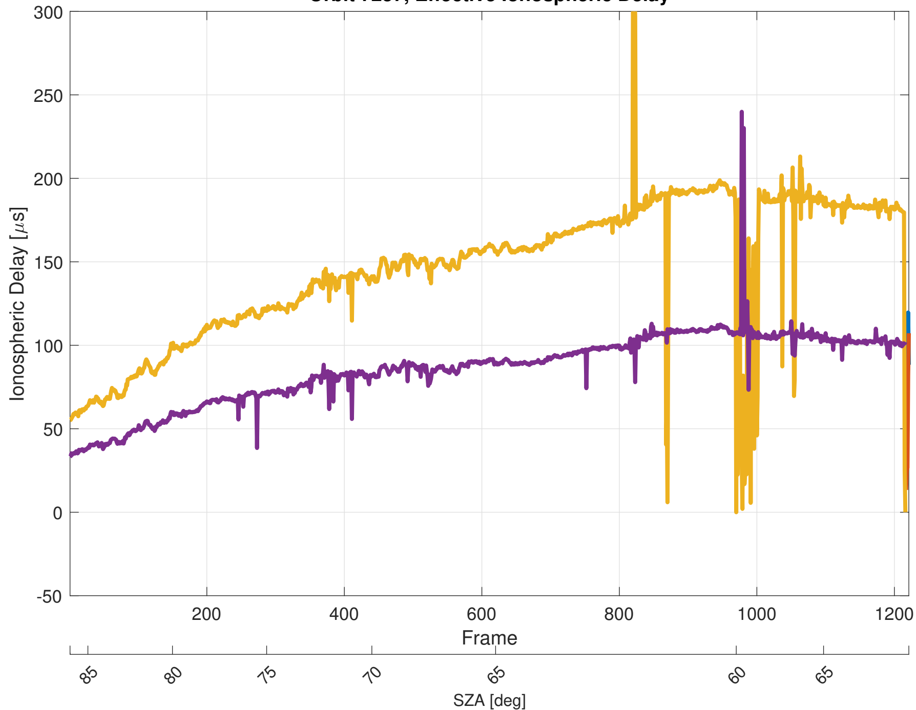
Orbit 7257, Effective Ionospheric Delay
