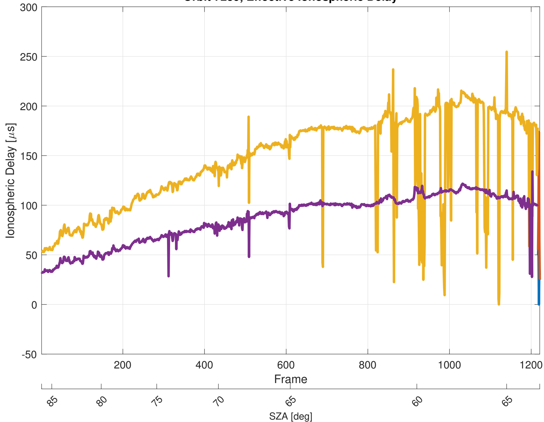
Orbit 7259, Effective Ionospheric Delay
