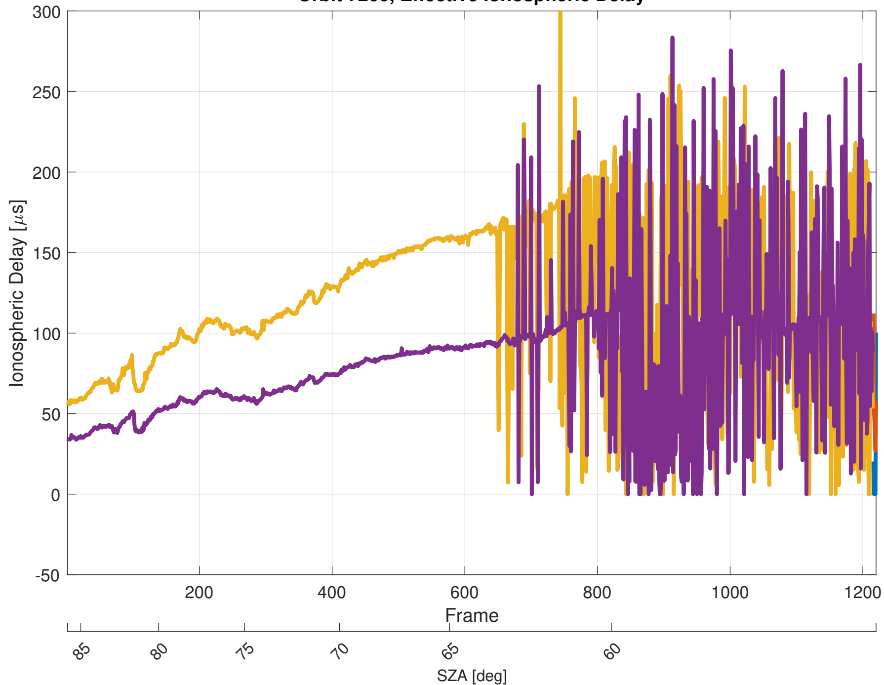
Orbit 7266, Effective Ionospheric Delay
