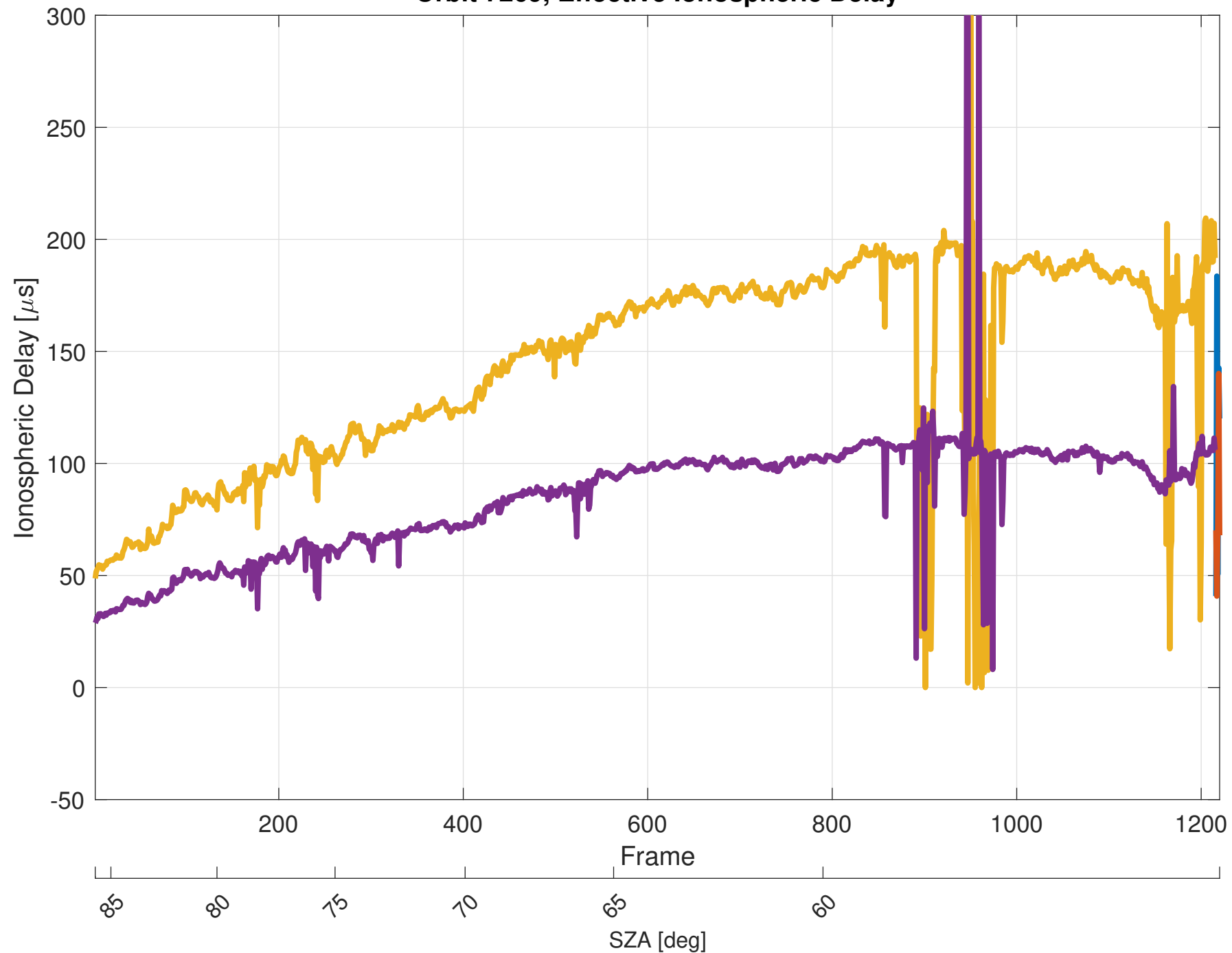
Orbit 7269, Effective Ionospheric Delay
