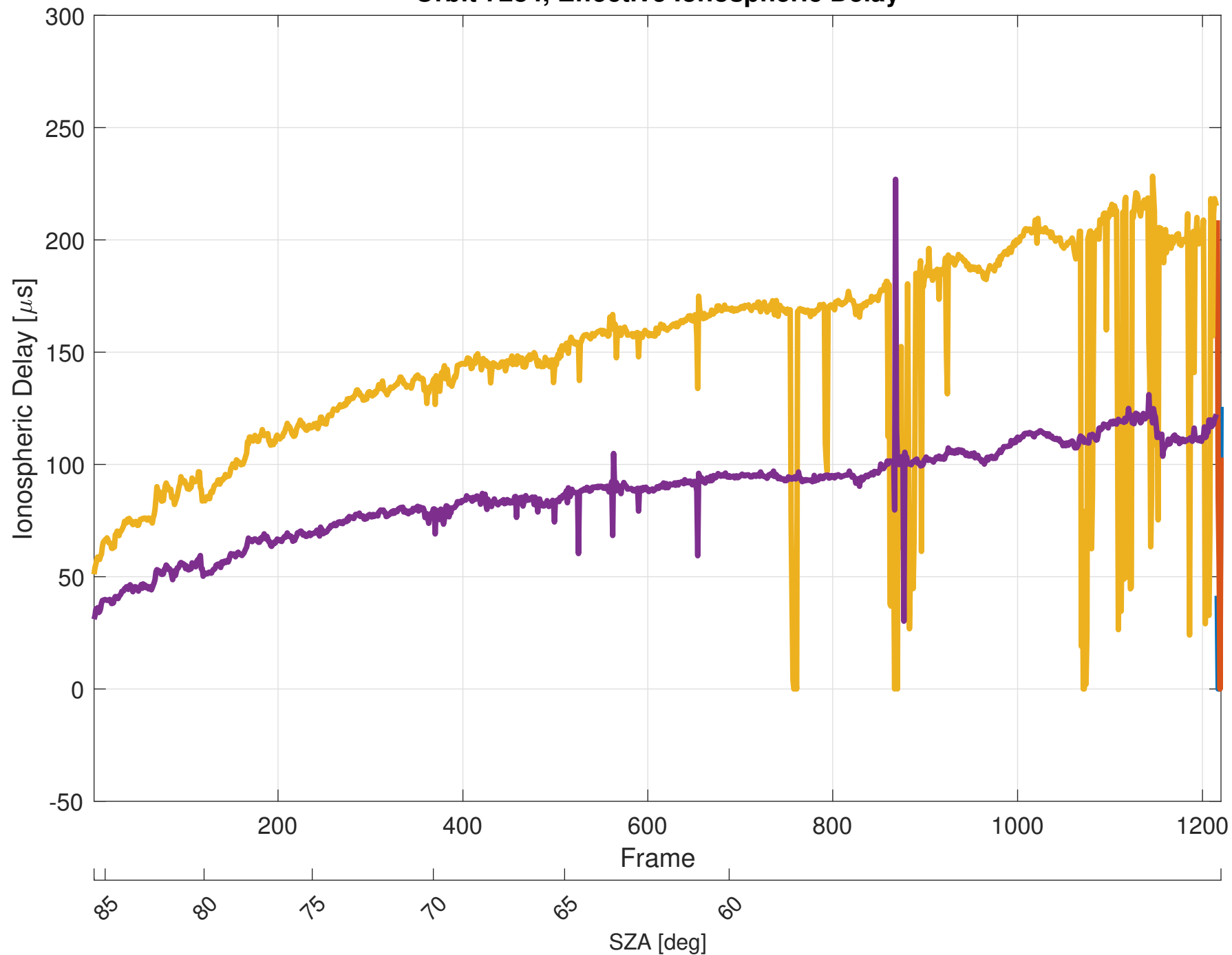
Orbit 7284, Effective Ionospheric Delay
