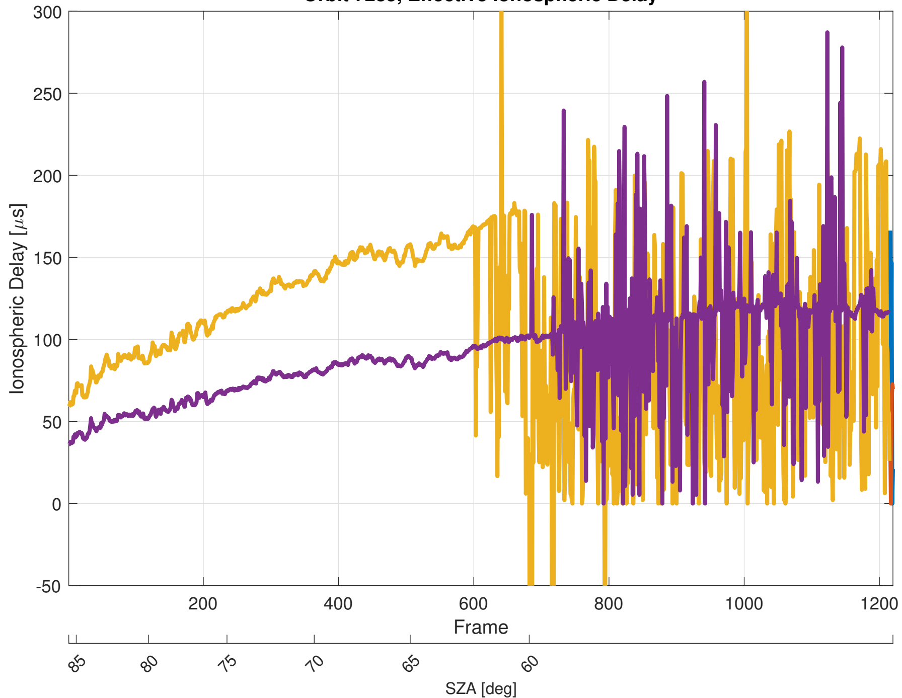
Orbit 7285, Effective Ionospheric Delay
