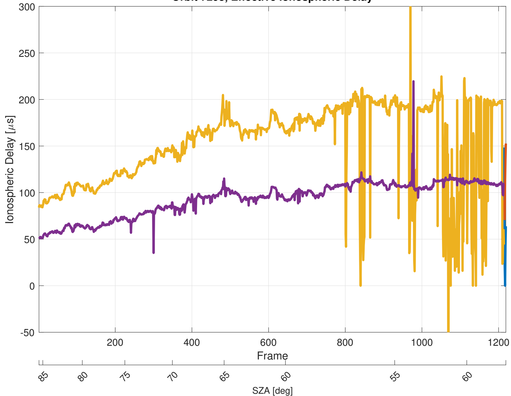
Orbit 7293, Effective Ionospheric Delay
