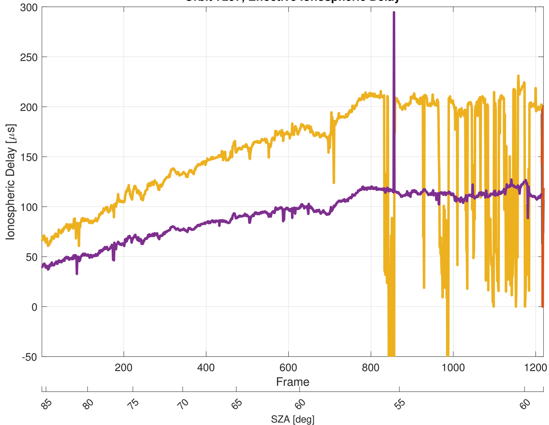
Orbit 7297, Effective Ionospheric Delay
