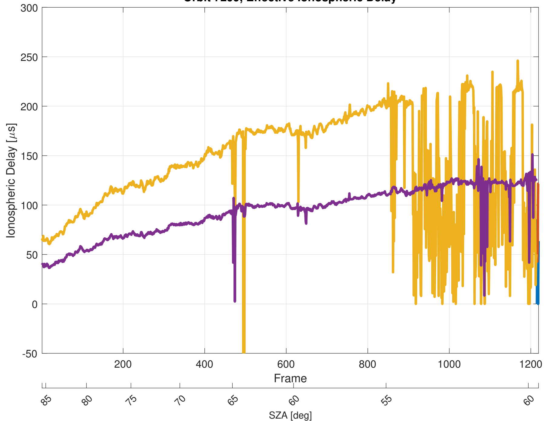
Orbit 7299, Effective Ionospheric Delay
