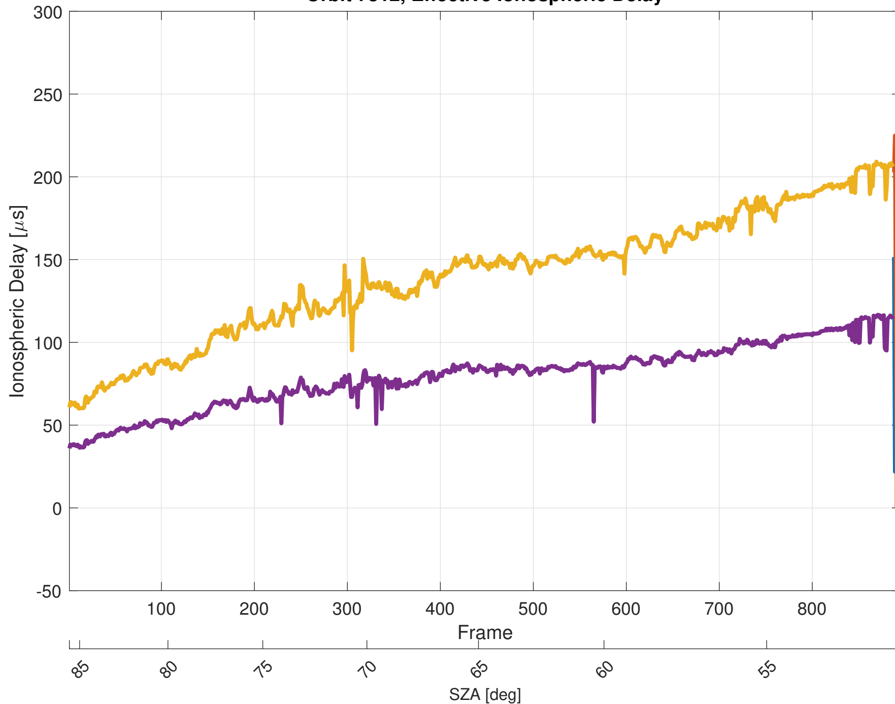
Orbit 7312, Effective Ionospheric Delay
