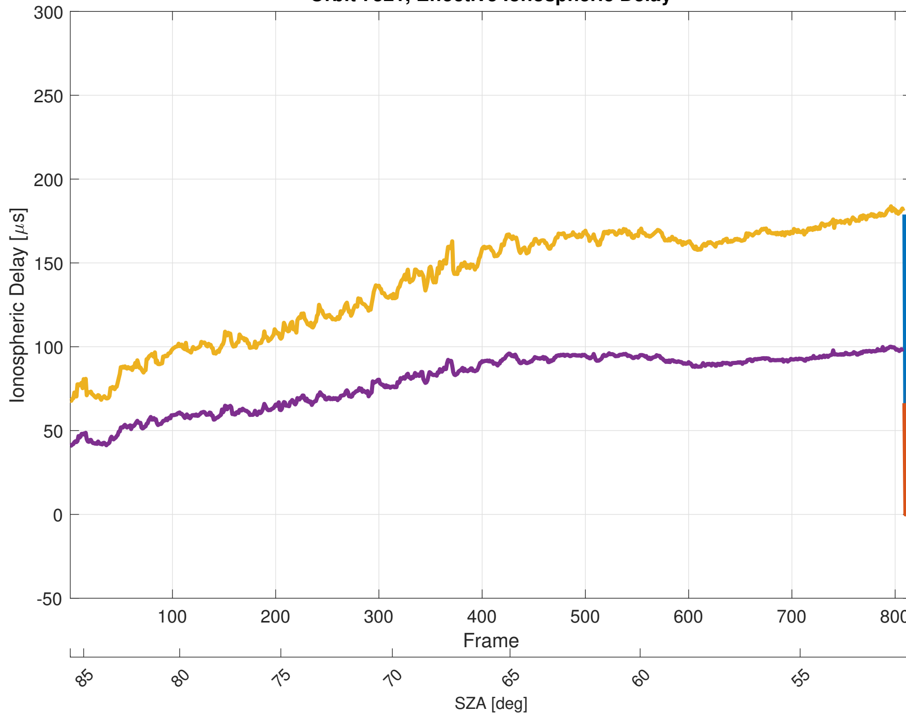
Orbit 7321, Effective Ionospheric Delay
