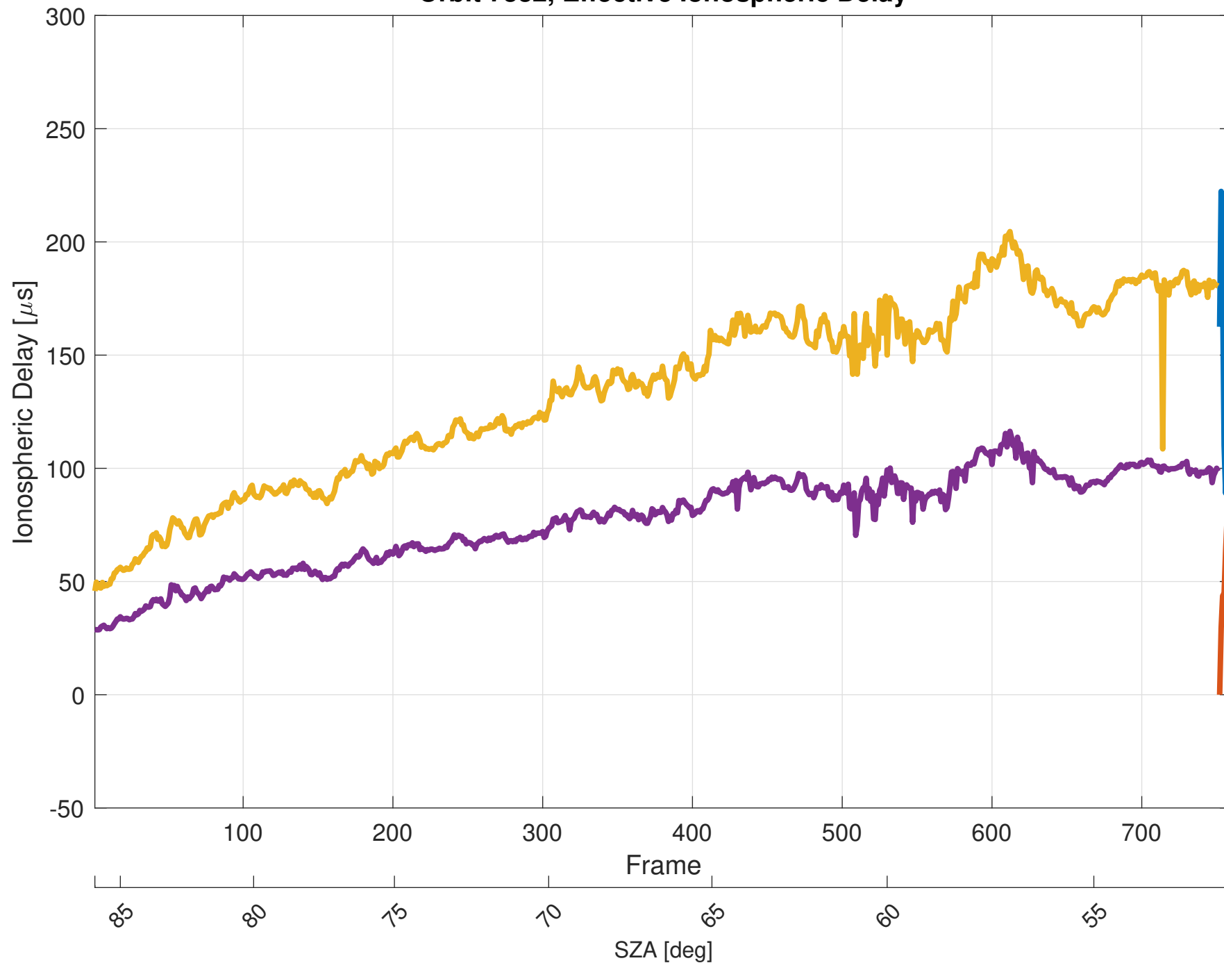
Orbit 7332, Effective Ionospheric Delay
