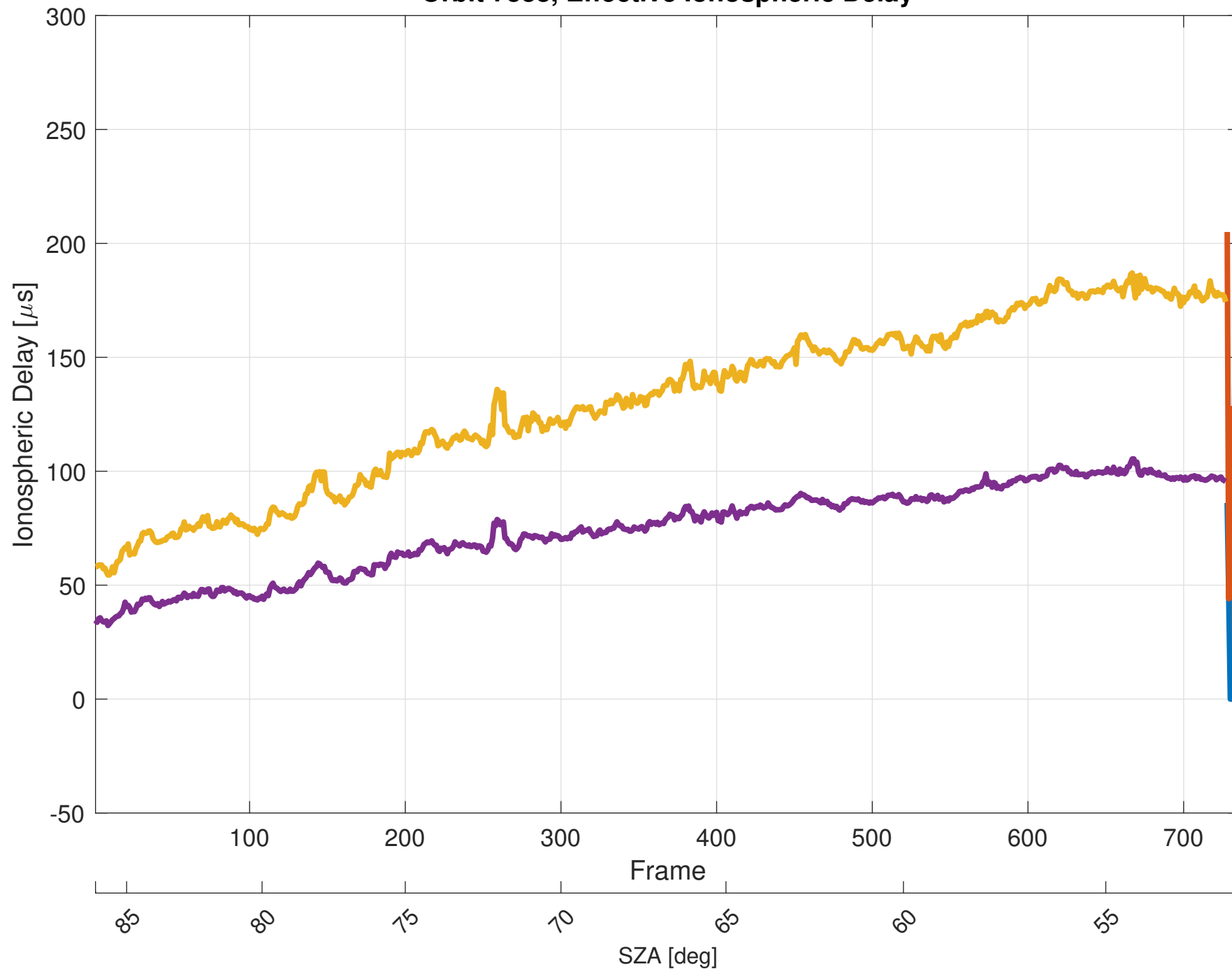
Orbit 7338, Effective Ionospheric Delay
