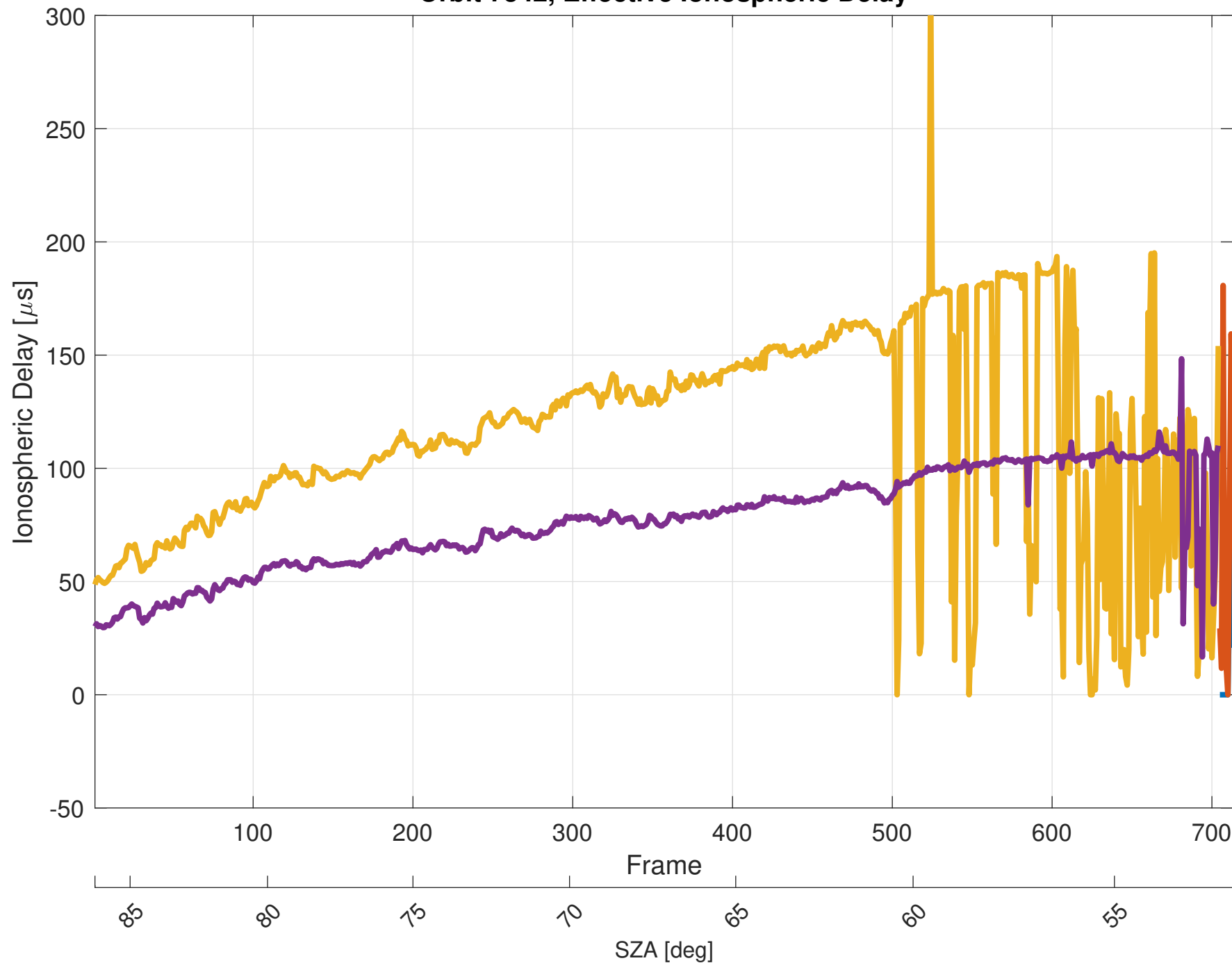
Orbit 7342, Effective Ionospheric Delay
