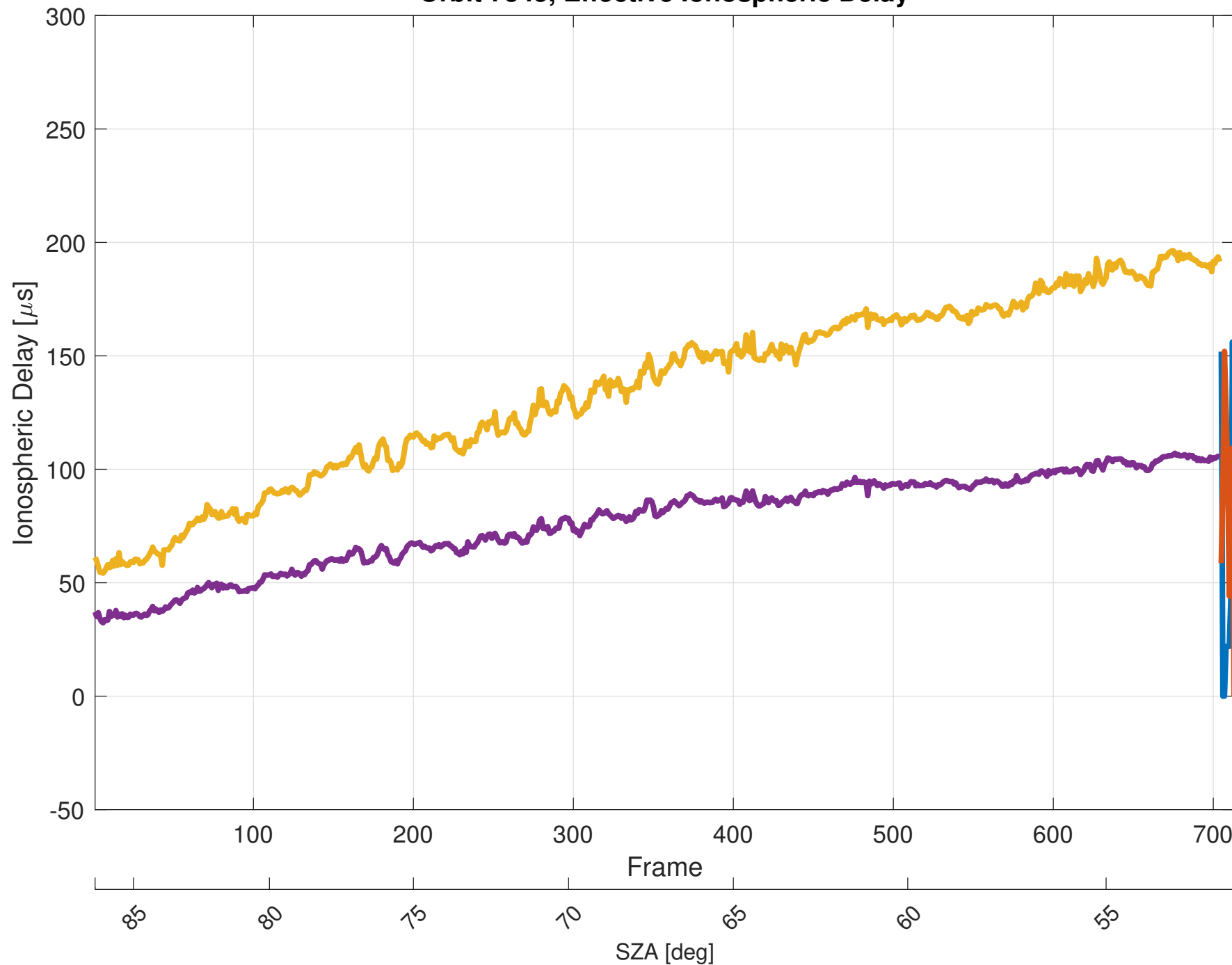
Orbit 7345, Effective Ionospheric Delay
