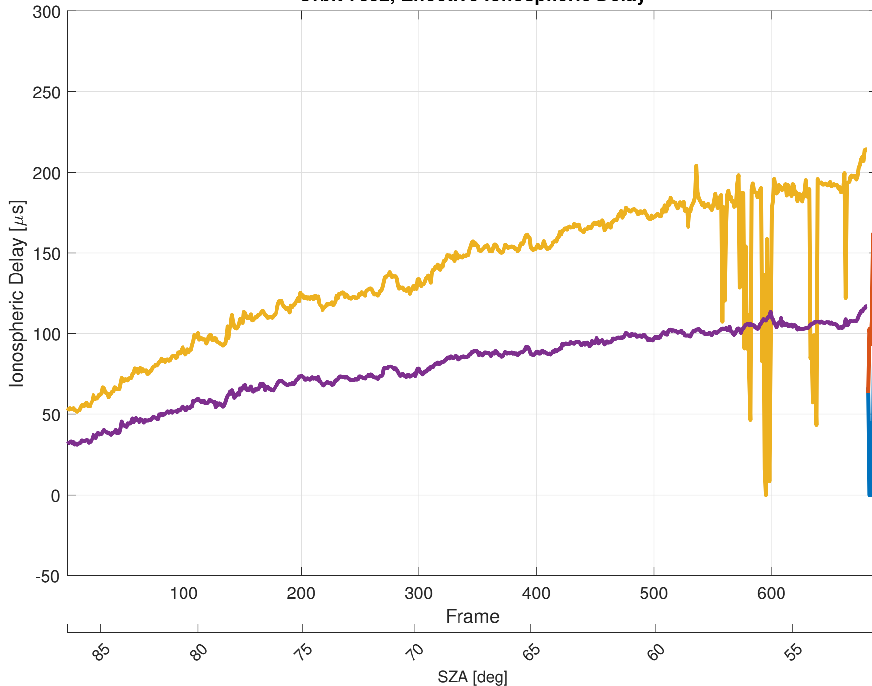
Orbit 7352, Effective Ionospheric Delay
