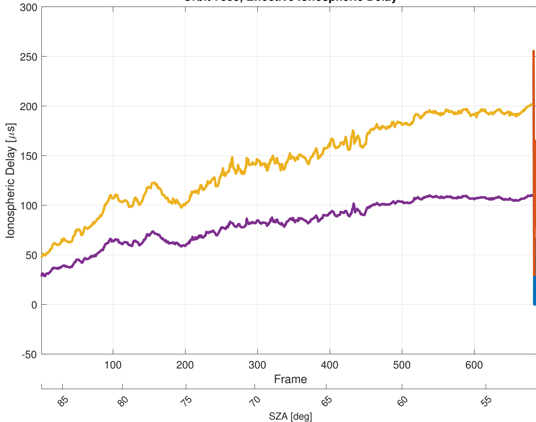
Orbit 7353, Effective Ionospheric Delay
