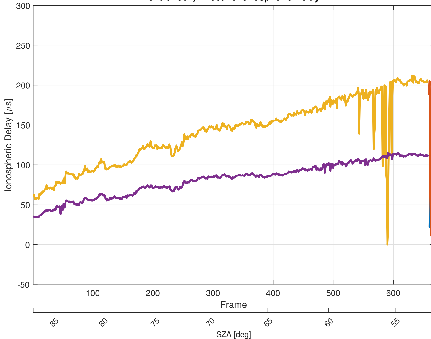
Orbit 7361, Effective Ionospheric Delay
