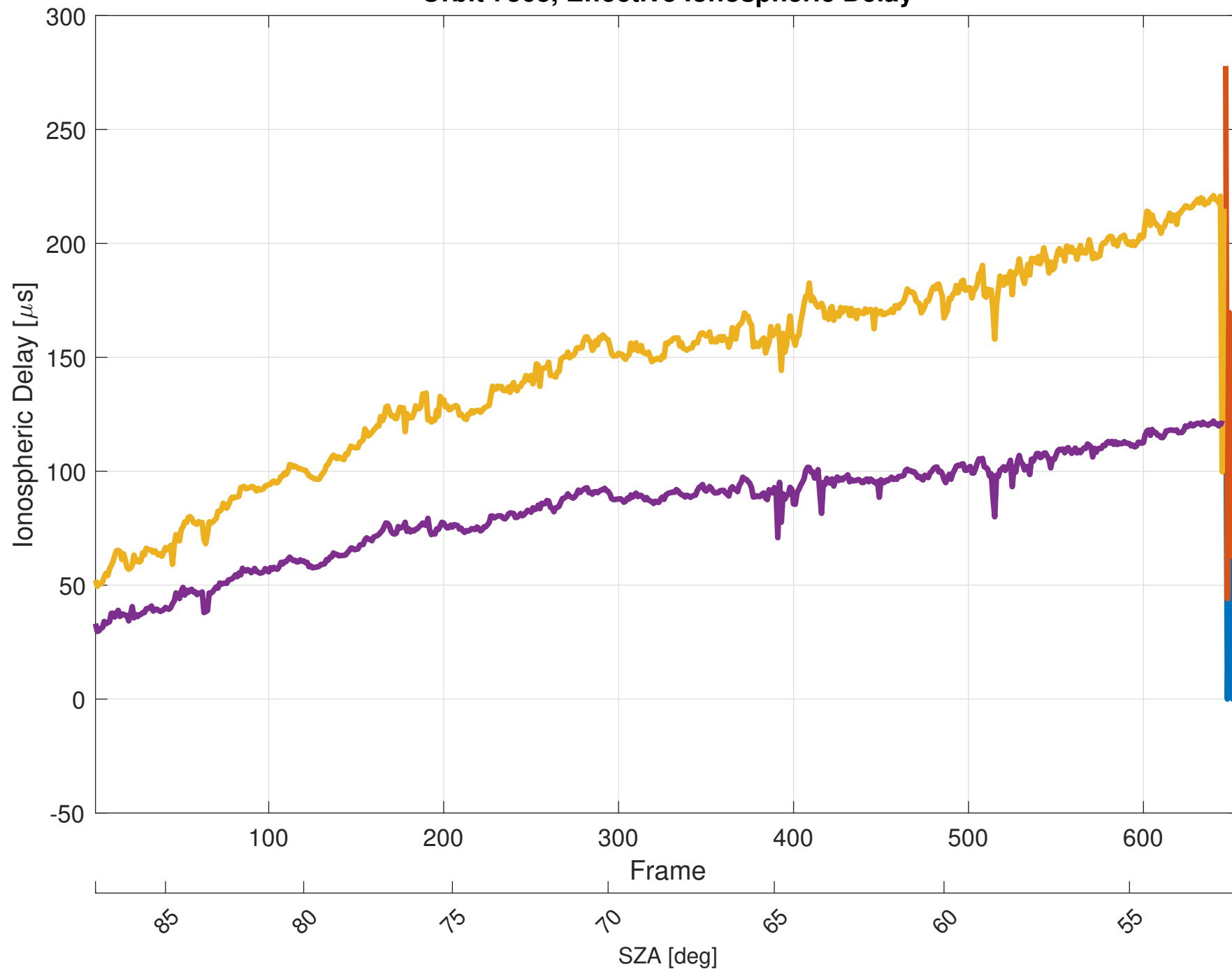
Orbit 7368, Effective Ionospheric Delay
