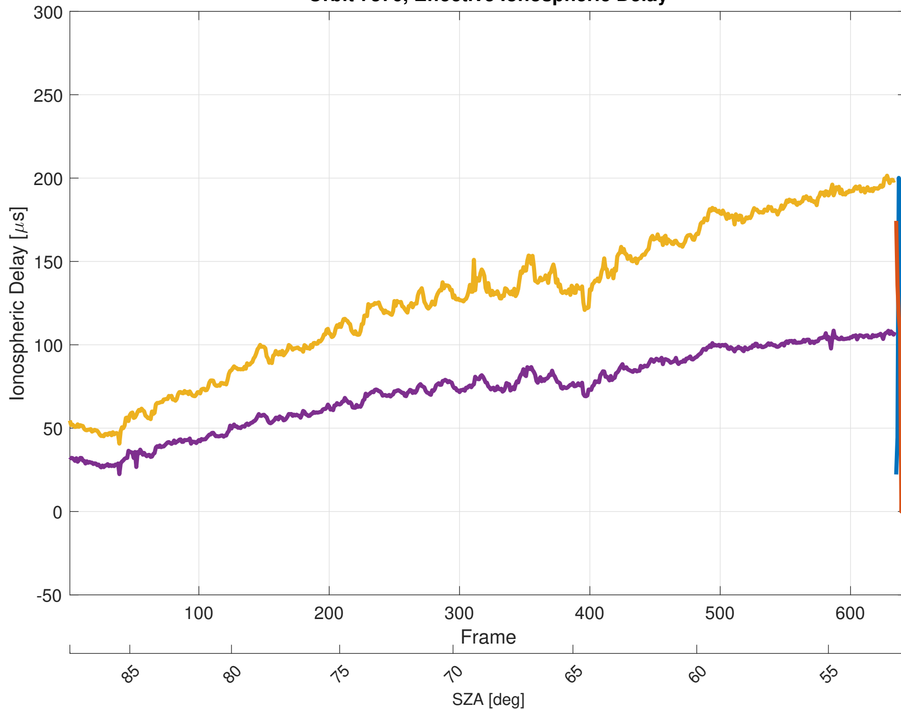
Orbit 7376, Effective Ionospheric Delay
