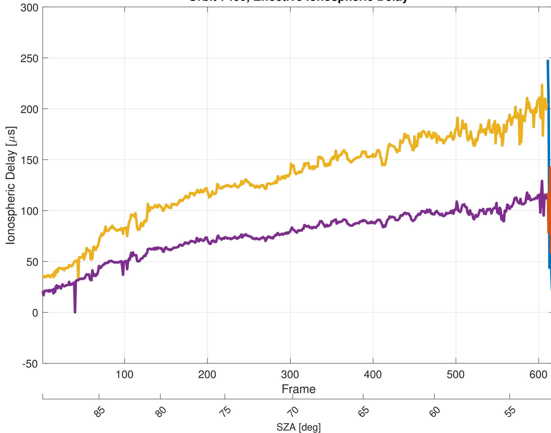
Orbit 7400, Effective Ionospheric Delay
