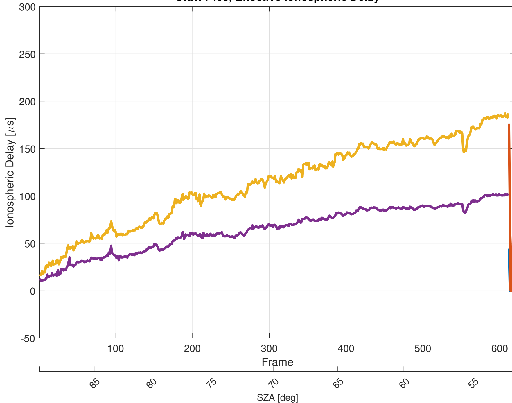
Orbit 7403, Effective Ionospheric Delay
