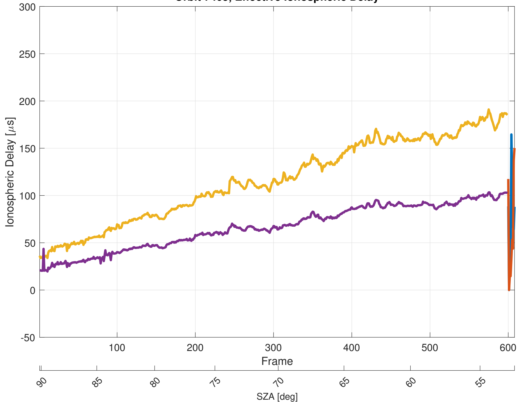
Orbit 7405, Effective Ionospheric Delay
