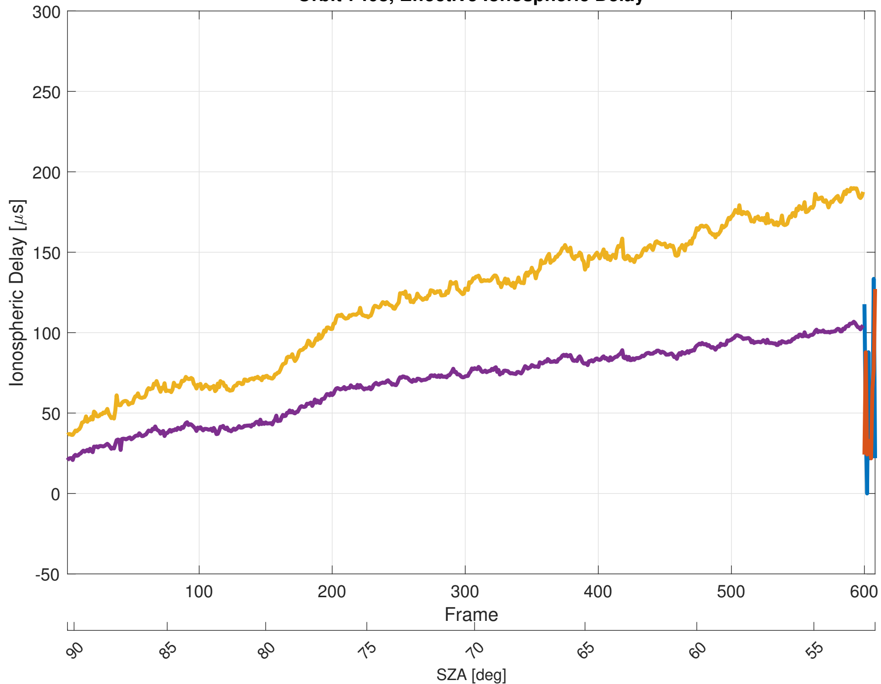
Orbit 7408, Effective Ionospheric Delay
