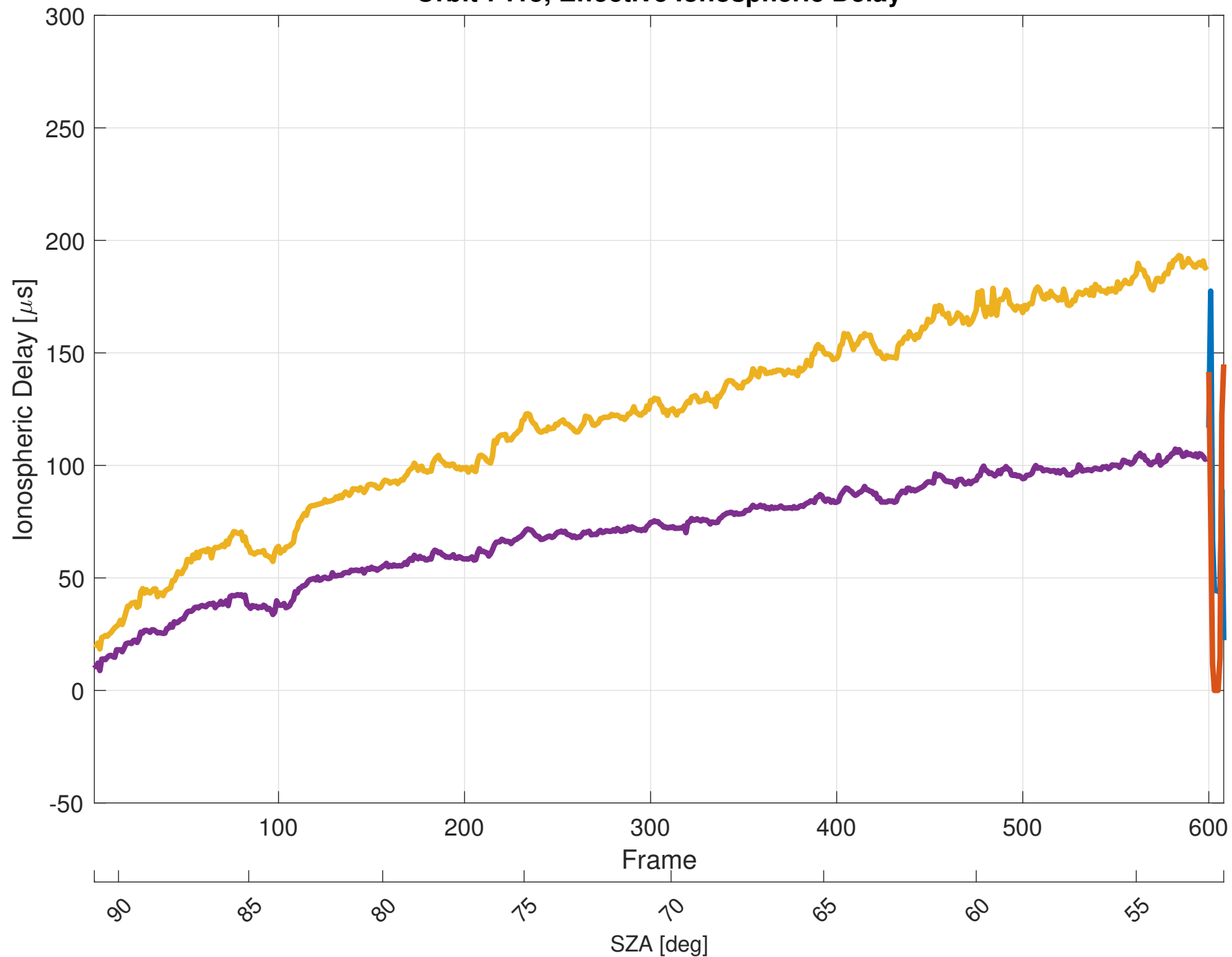
Orbit 7415, Effective Ionospheric Delay
