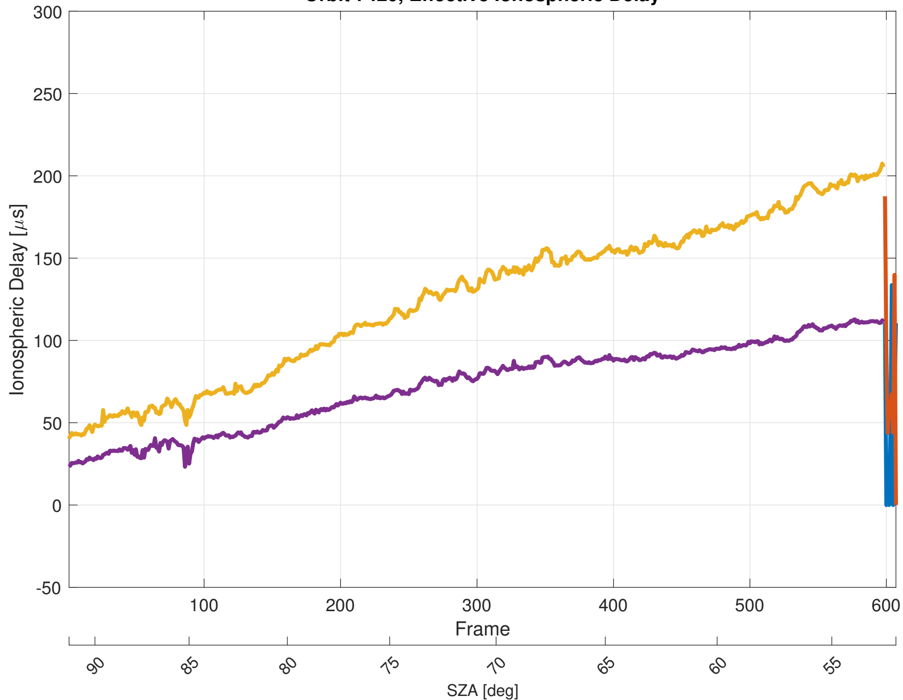
Orbit 7420, Effective Ionospheric Delay
