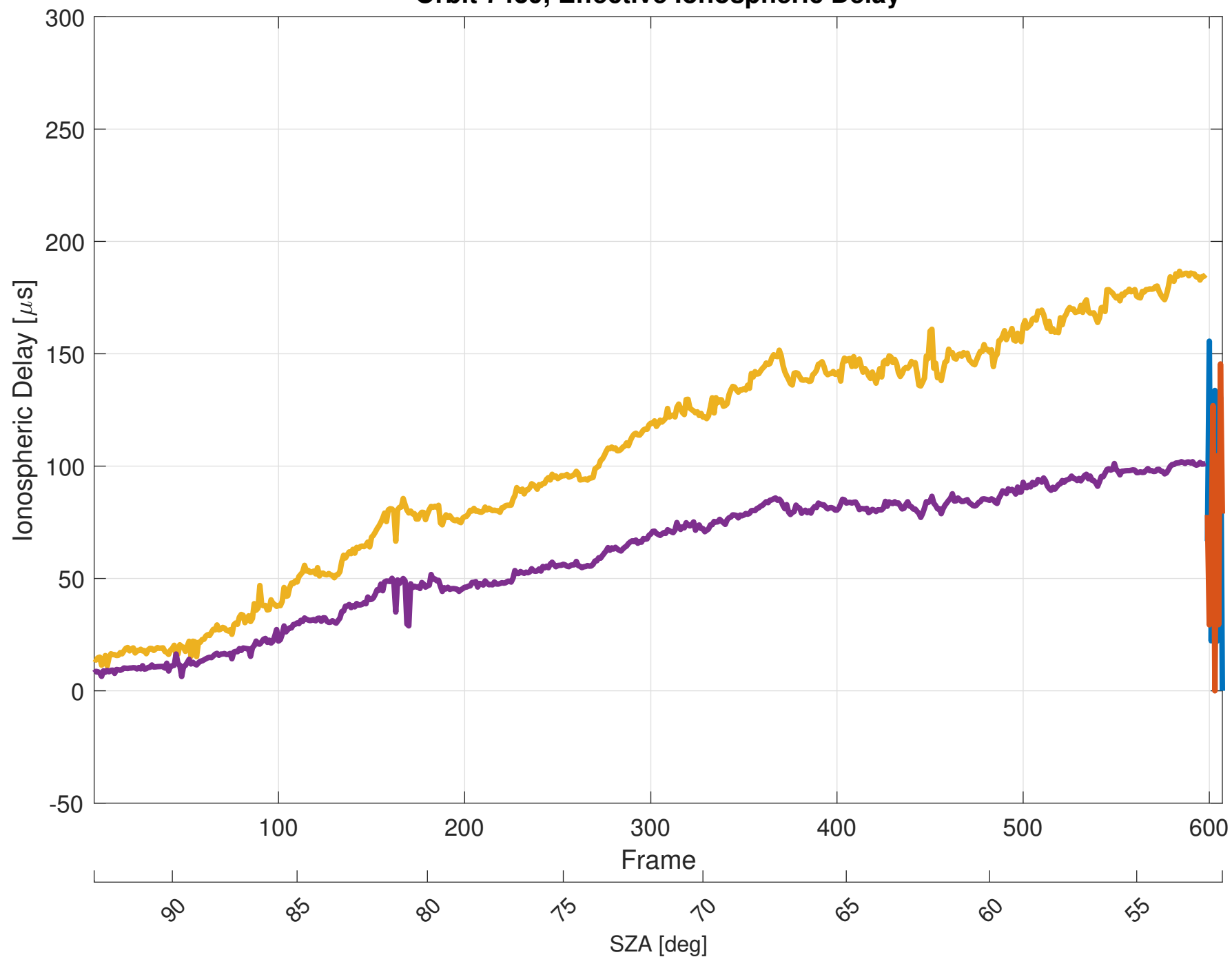
Orbit 7439, Effective Ionospheric Delay
