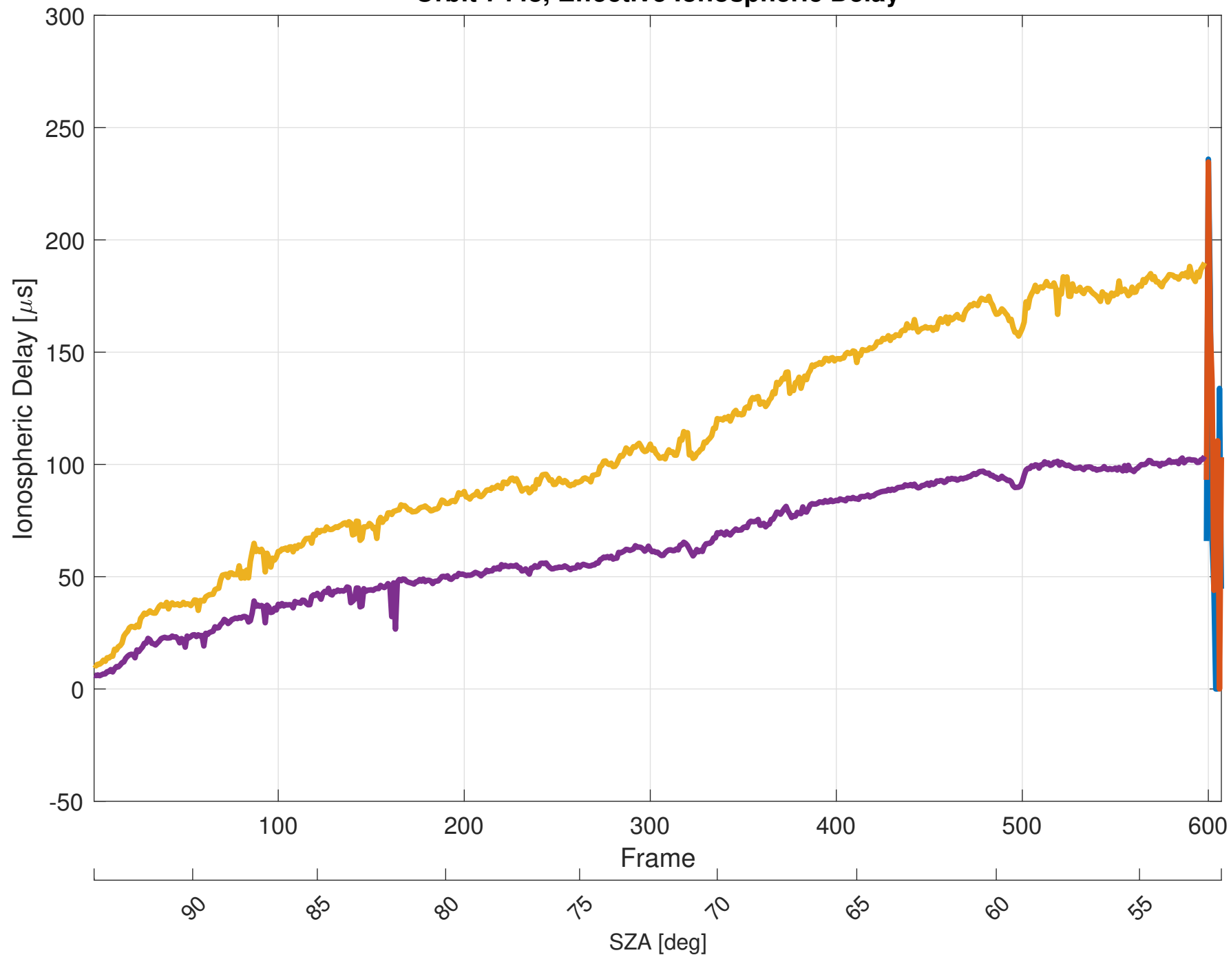
Orbit 7448, Effective Ionospheric Delay
