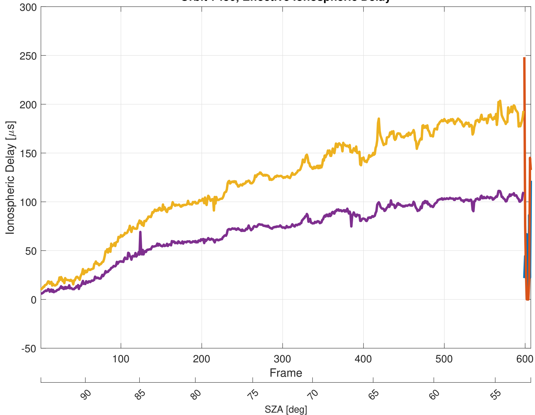
Orbit 7450, Effective Ionospheric Delay
