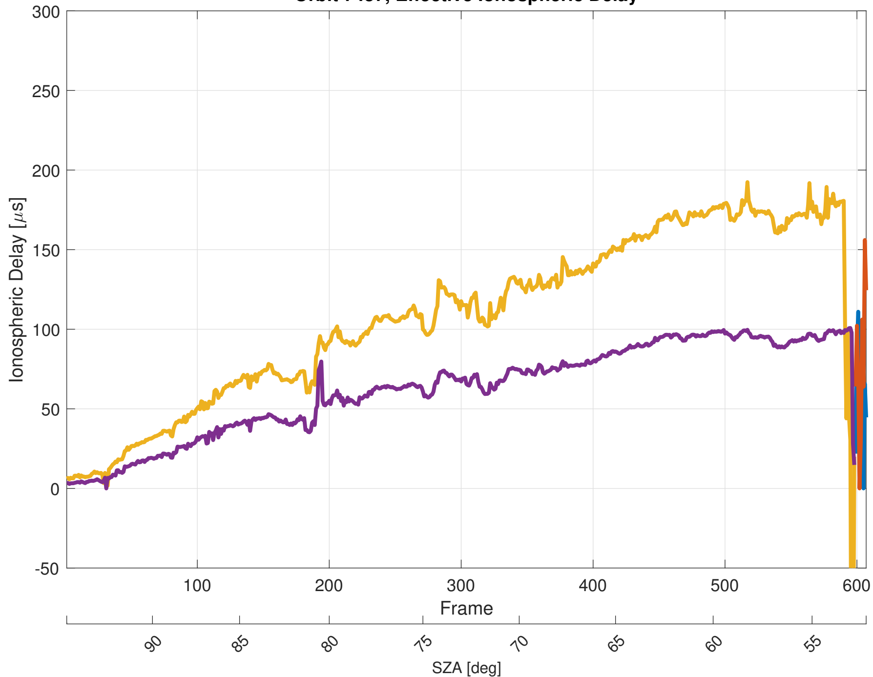
Orbit 7457, Effective Ionospheric Delay
