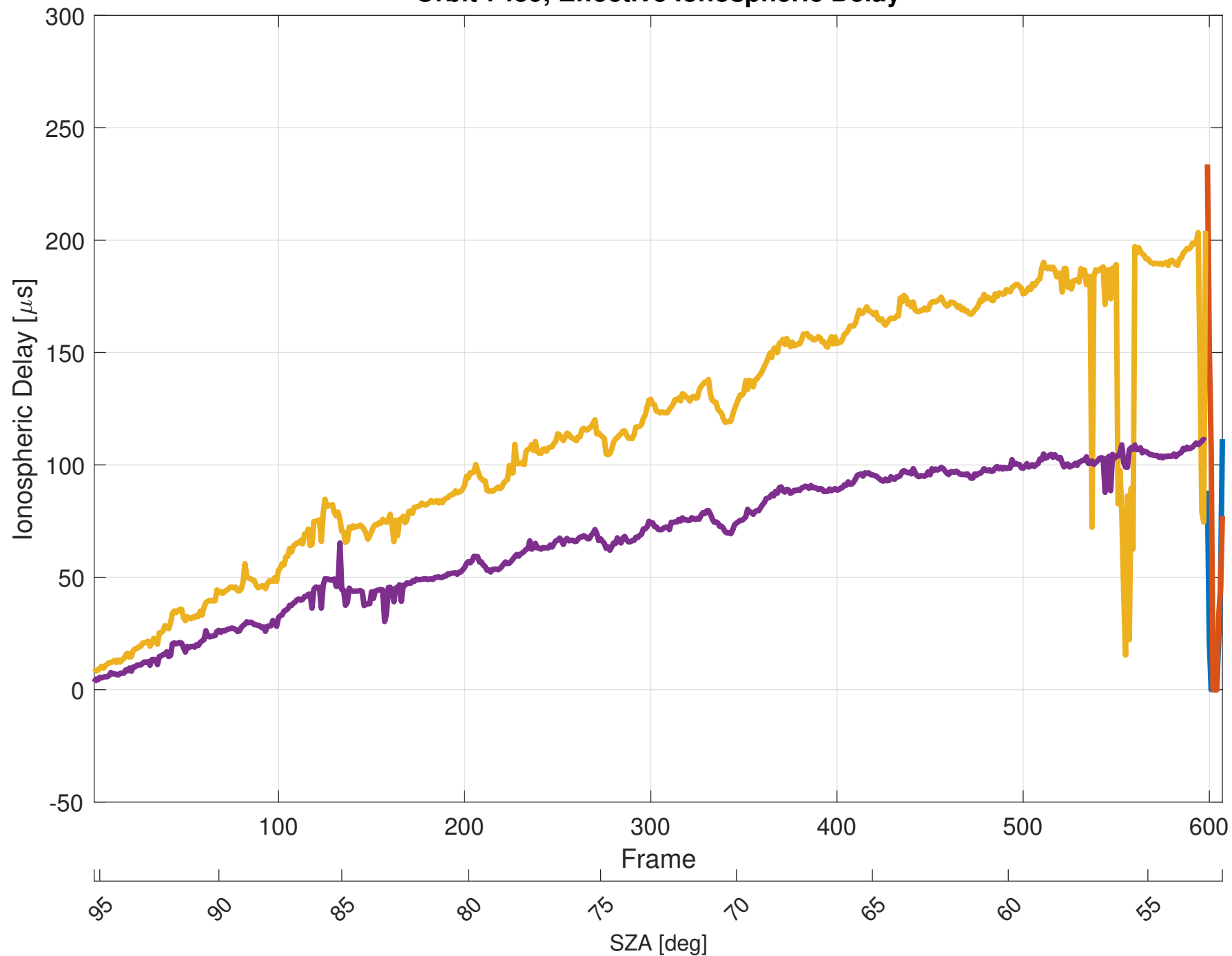
Orbit 7459, Effective Ionospheric Delay
