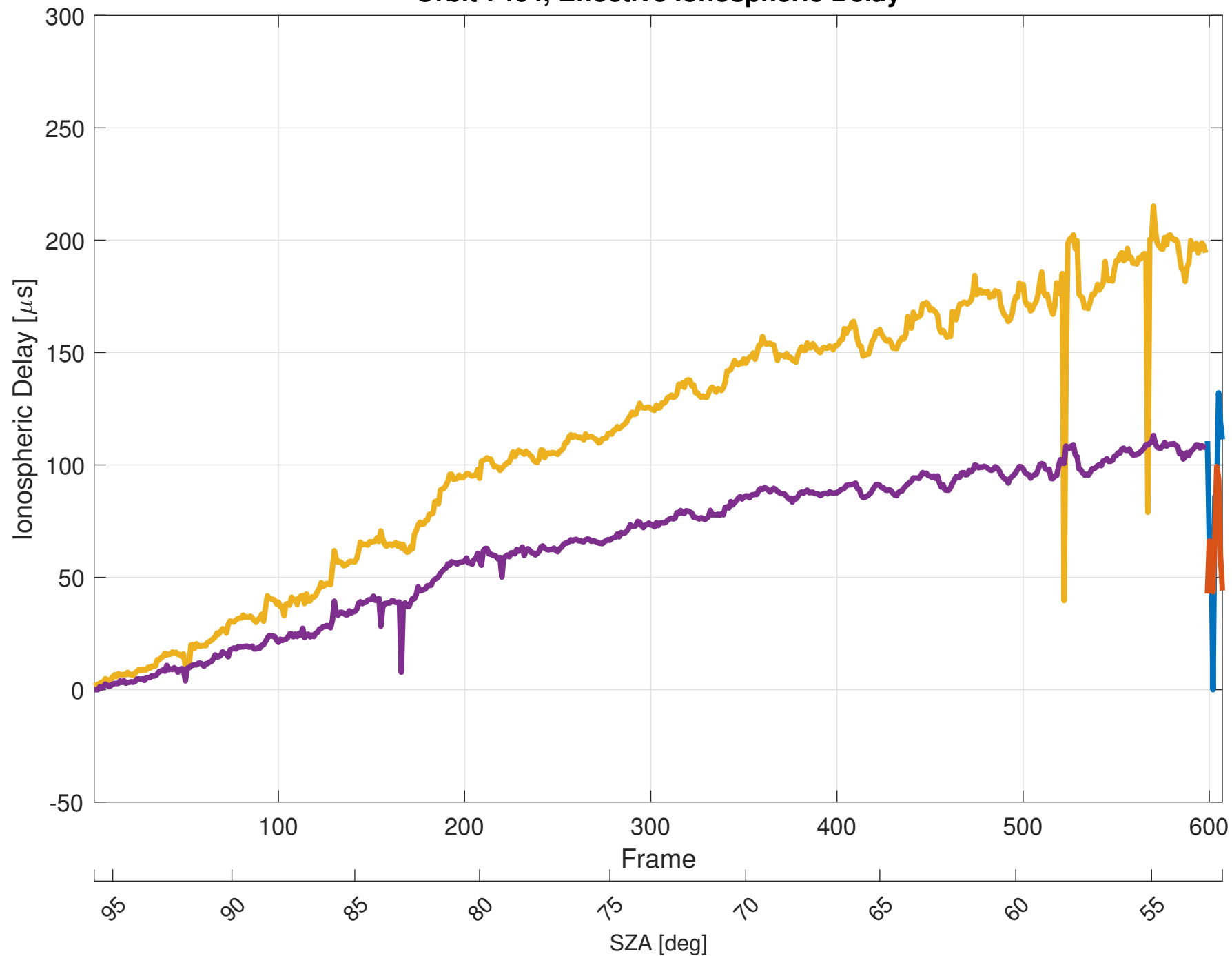
Orbit 7464, Effective Ionospheric Delay
