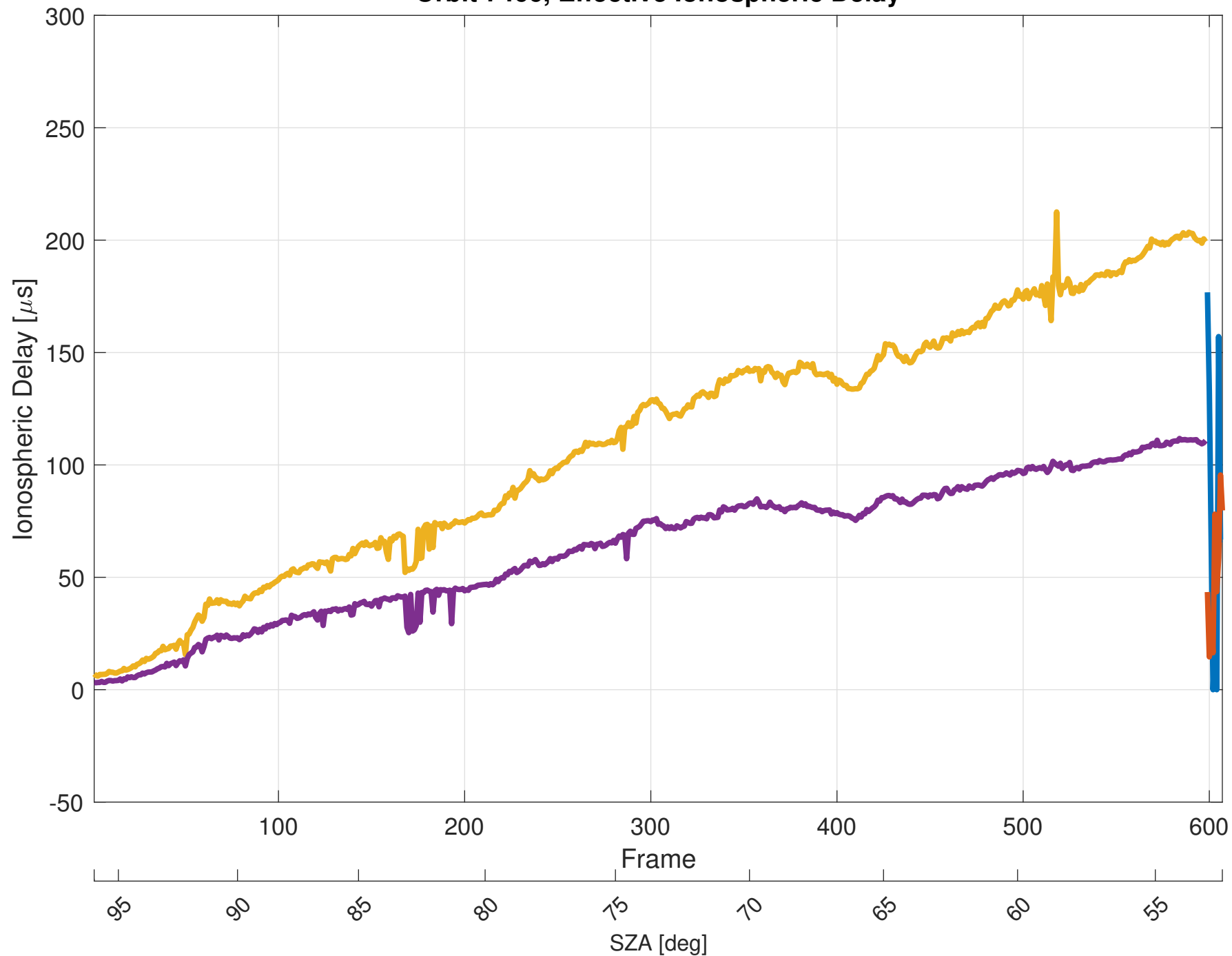
Orbit 7466, Effective Ionospheric Delay
