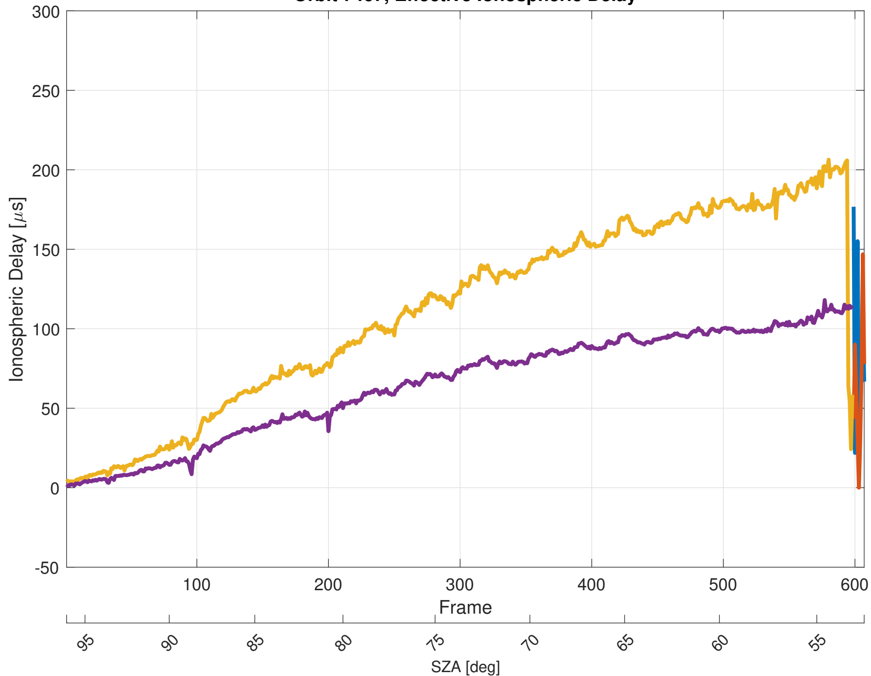
Orbit 7467, Effective Ionospheric Delay
