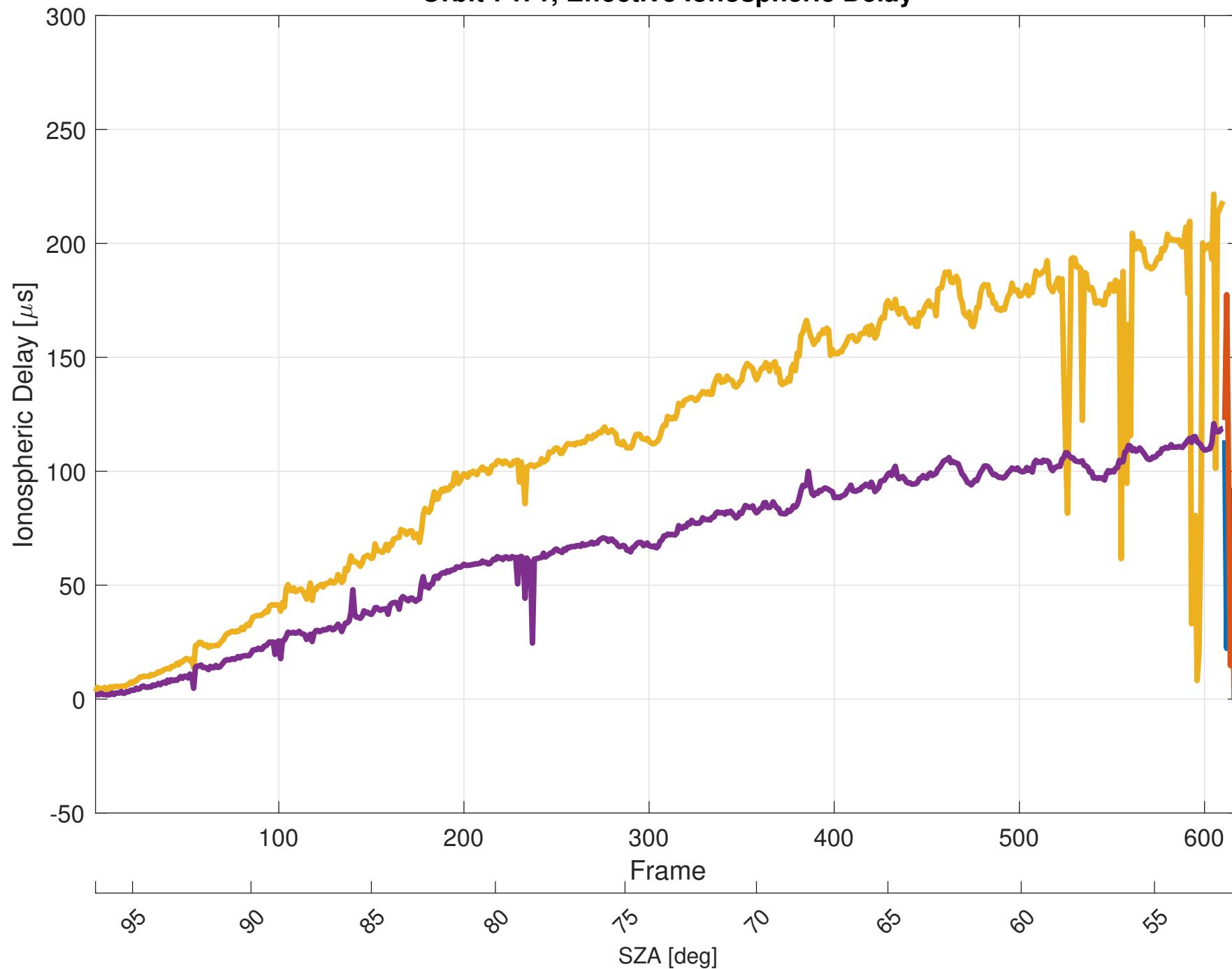
Orbit 7471, Effective Ionospheric Delay
