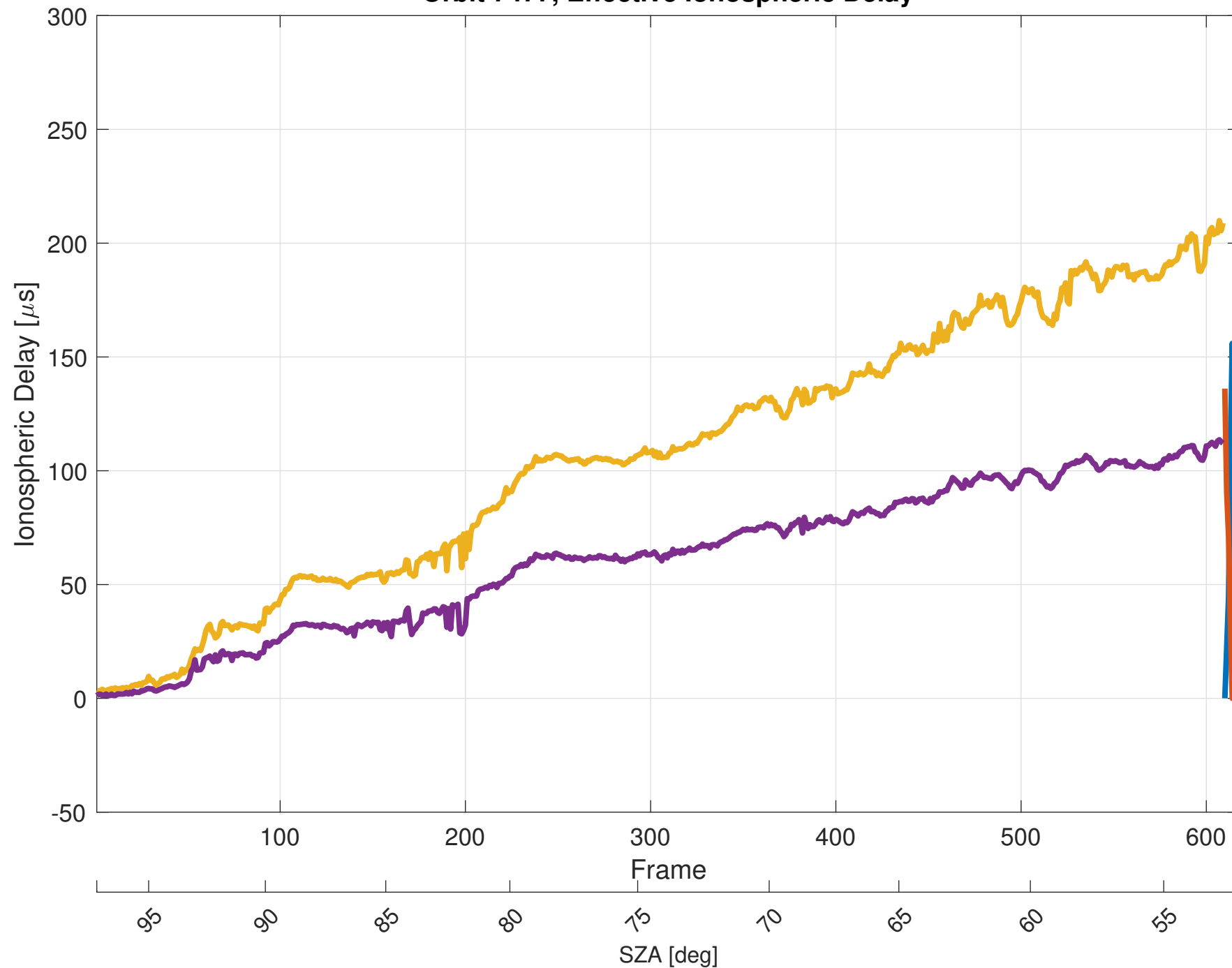
Orbit 7477, Effective Ionospheric Delay
