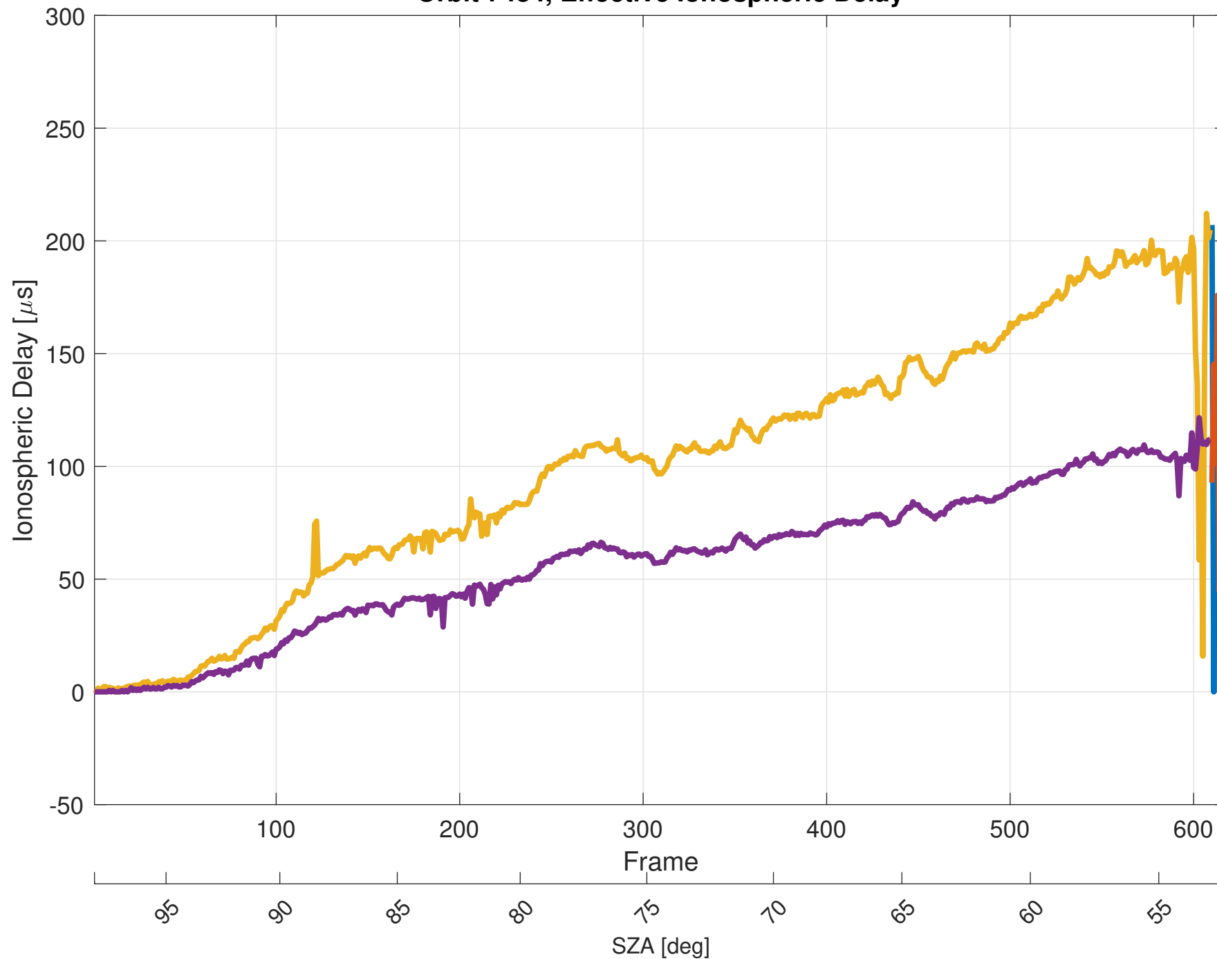
Orbit 7484, Effective Ionospheric Delay
