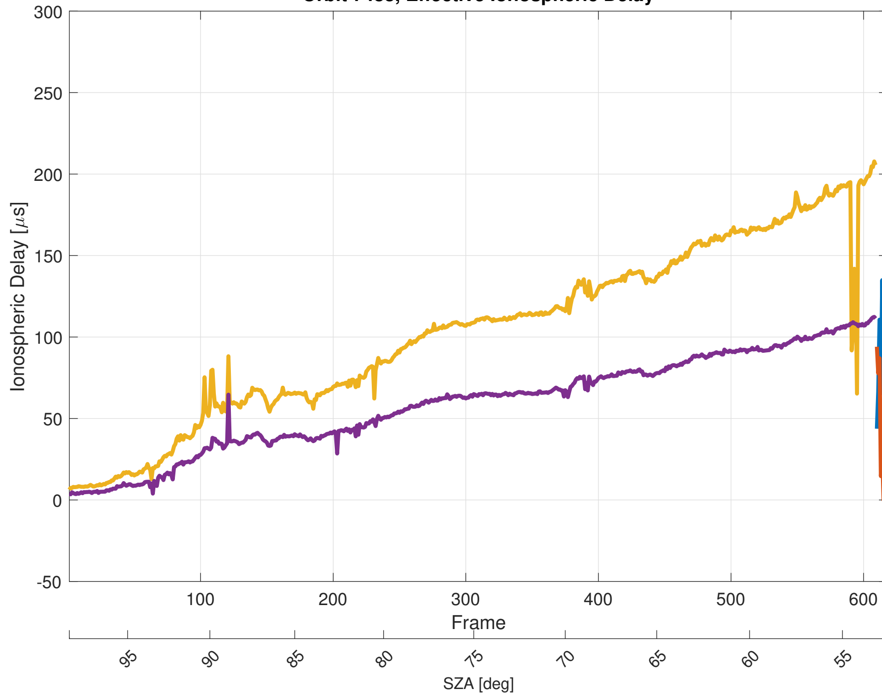
Orbit 7488, Effective Ionospheric Delay
