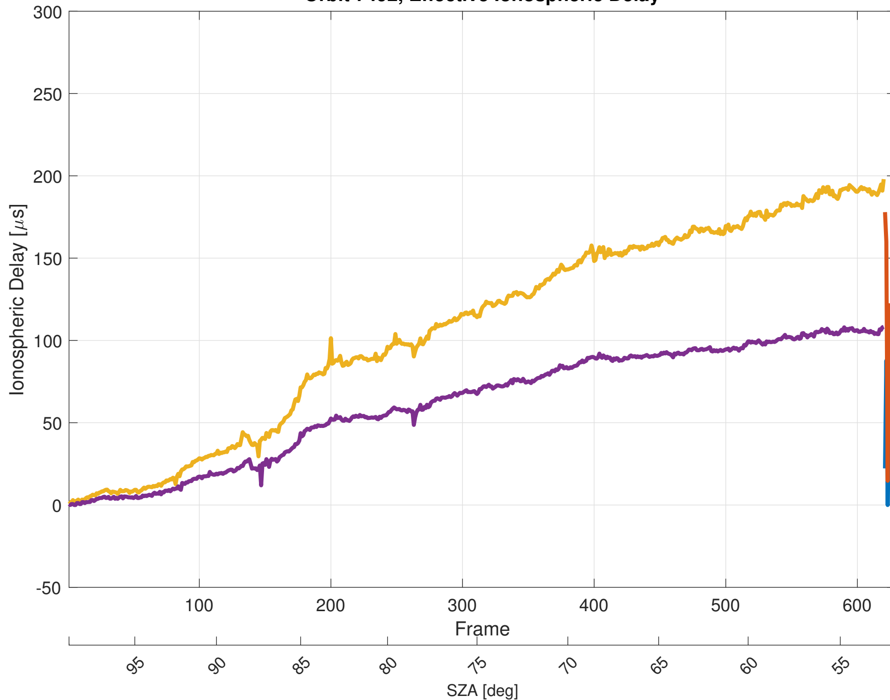
Orbit 7492, Effective Ionospheric Delay
