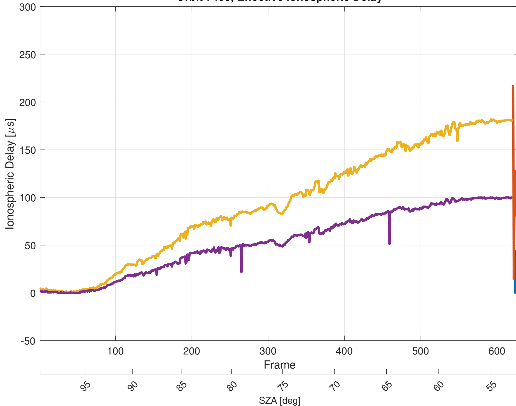
Orbit 7498, Effective Ionospheric Delay
