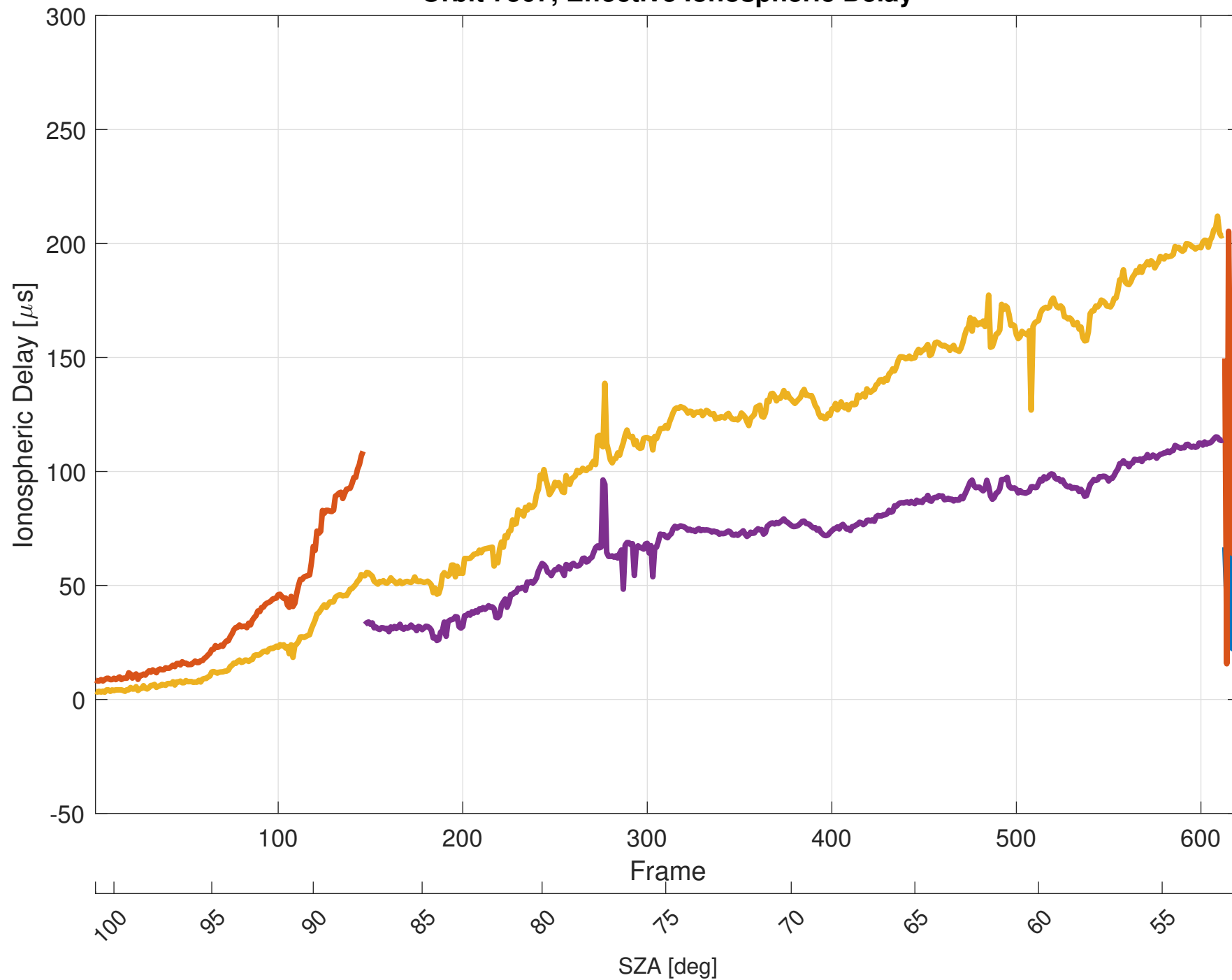
Orbit 7507, Effective Ionospheric Delay
